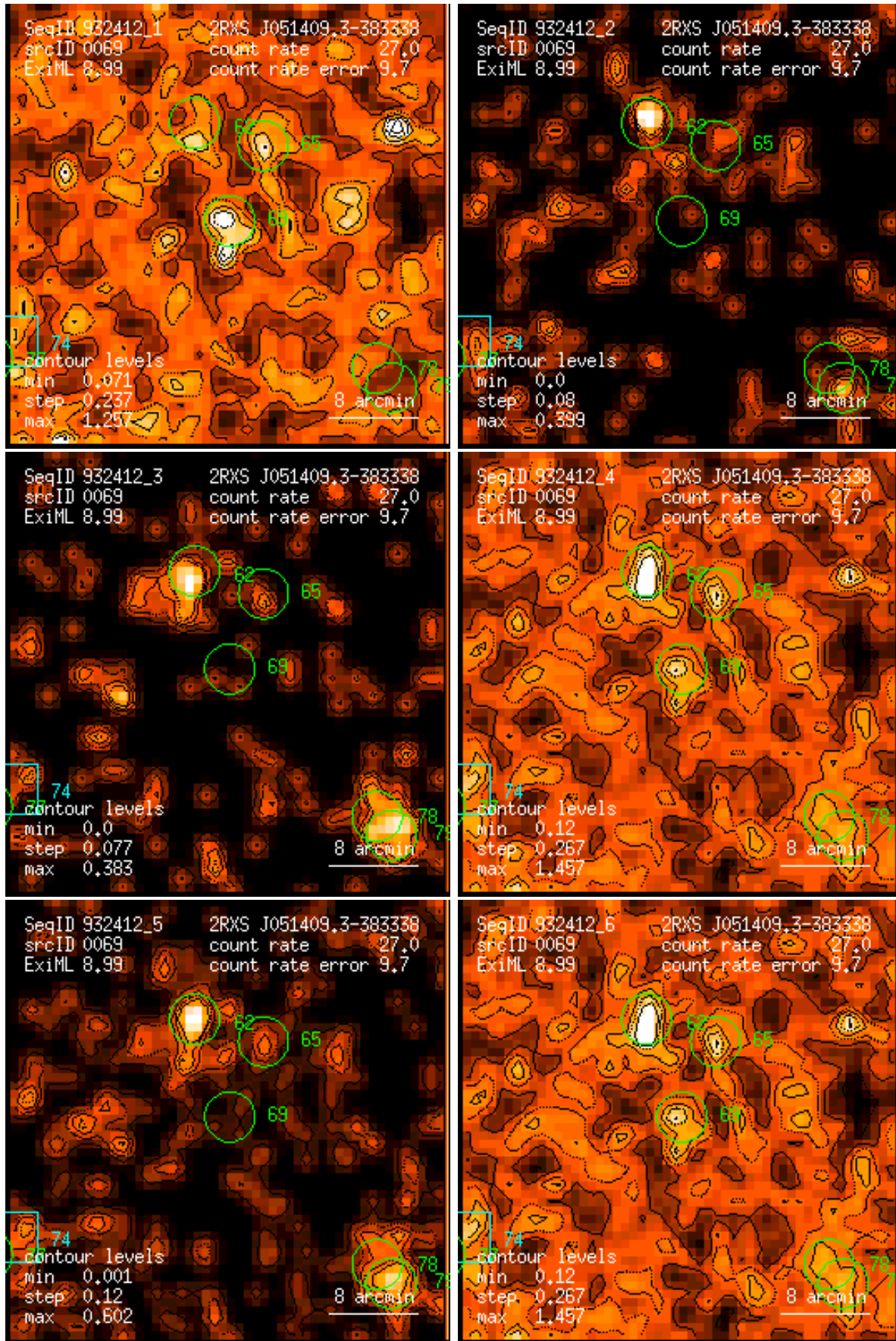
Figure 69: RASS 932412: detection 0069: band rate images, Gaussian filter: (1) PSPC channels 11 – 41, (2) 52 – 90, (3) 91 – 201, (4) 11 – 235, (5) 52 – 201, (6) 11 – 201. Broad band rates in counts/ks. Band rate contour levels in counts/ks/arcmin 2 .
