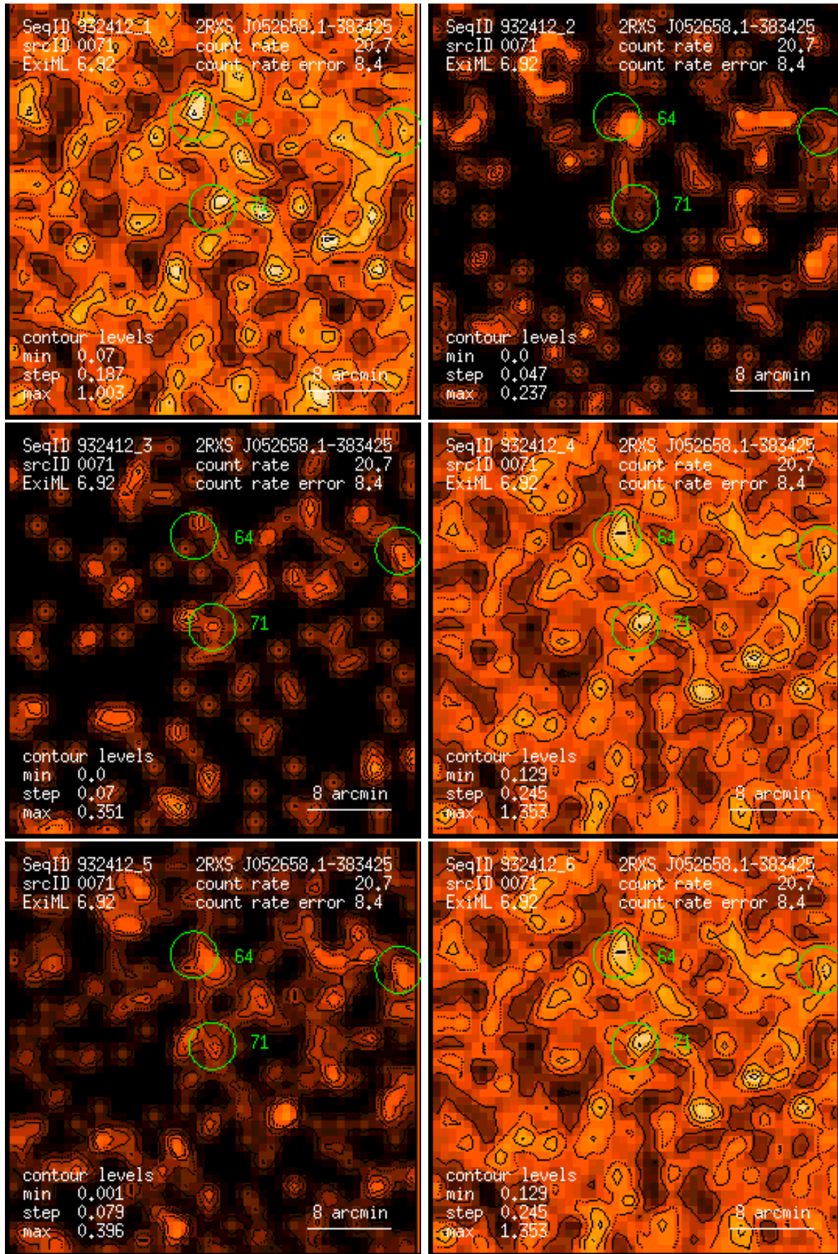
Figure 71: RASS 932412: detection 0071: band rate images, Gaussian filter: (1) PSPC channels 11 – 41, (2) 52 – 90, (3) 91 – 201, (4) 11 – 235, (5) 52 – 201, (6) 11 – 201. Broad band rates in counts/ks. Band rate contour levels in counts/ks/arcmin 2 .
