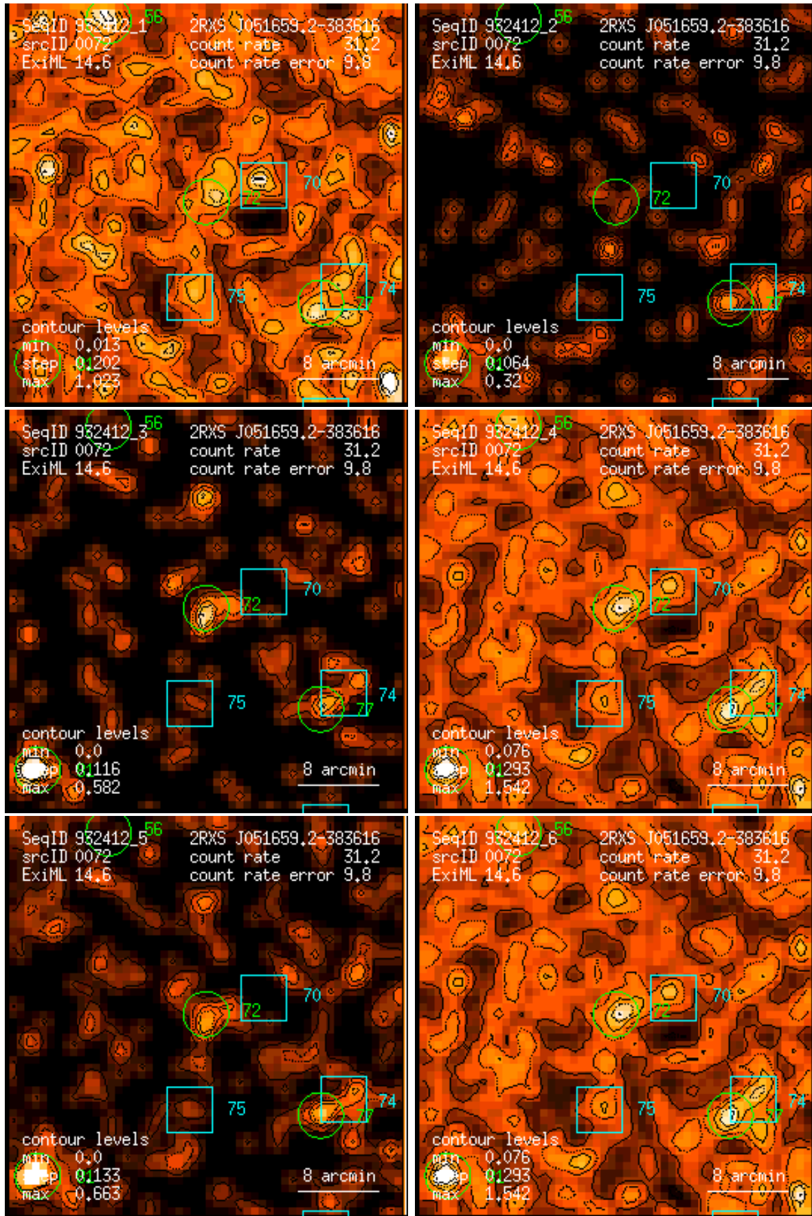
Figure 72: RASS 932412: detection 0072: band rate images, Gaussian filter: (1) PSPC channels 11 – 41, (2) 52 – 90, (3) 91 – 201, (4) 11 – 235, (5) 52 – 201, (6) 11 – 201. Broad band rates in counts/ks. Band rate contour levels in counts/ks/arcmin 2 .
