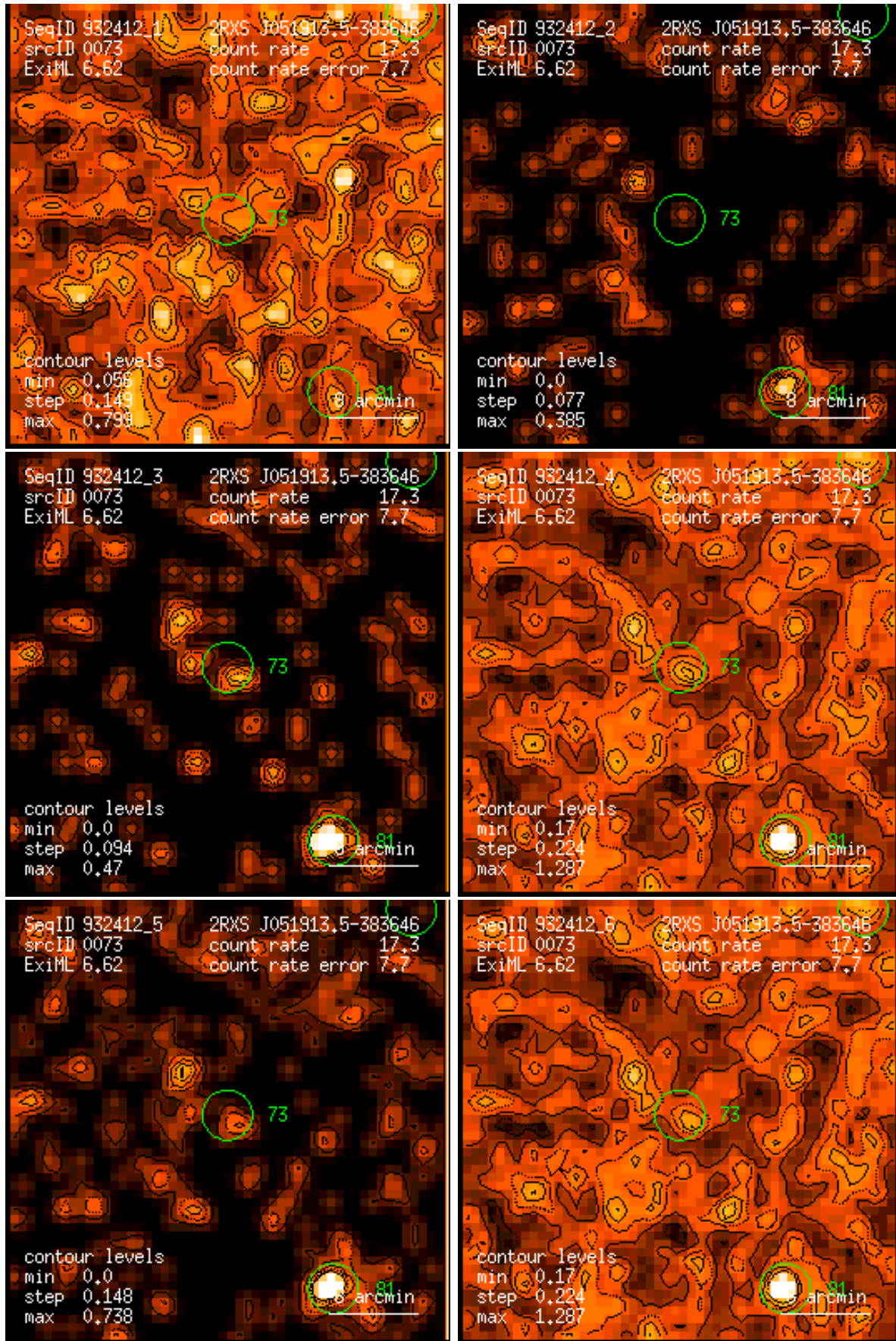
Figure 73: RASS 932412: detection 0073: band rate images, Gaussian filter: (1) PSPC channels 11 – 41, (2) 52 – 90, (3) 91 – 201, (4) 11 – 235, (5) 52 – 201, (6) 11 – 201. Broad band rates in counts/ks. Band rate contour levels in counts/ks/arcmin 2 .
