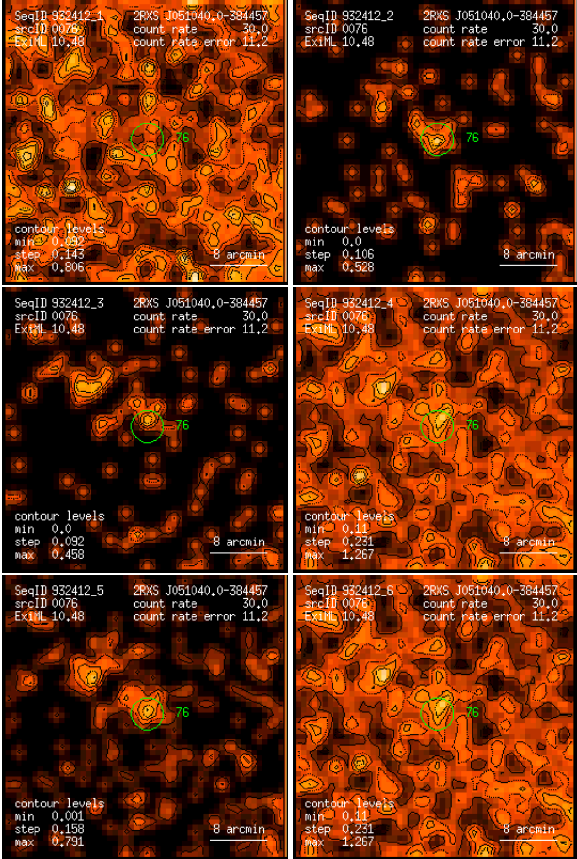
Figure 76: RASS 932412: detection 0076: band rate images, Gaussian filter: (1) PSPC channels 11 – 41, (2) 52 – 90, (3) 91 – 201, (4) 11 – 235, (5) 52 – 201, (6) 11 – 201. Broad band rates in counts/ks. Band rate contour levels in counts/ks/arcmin 2 .
