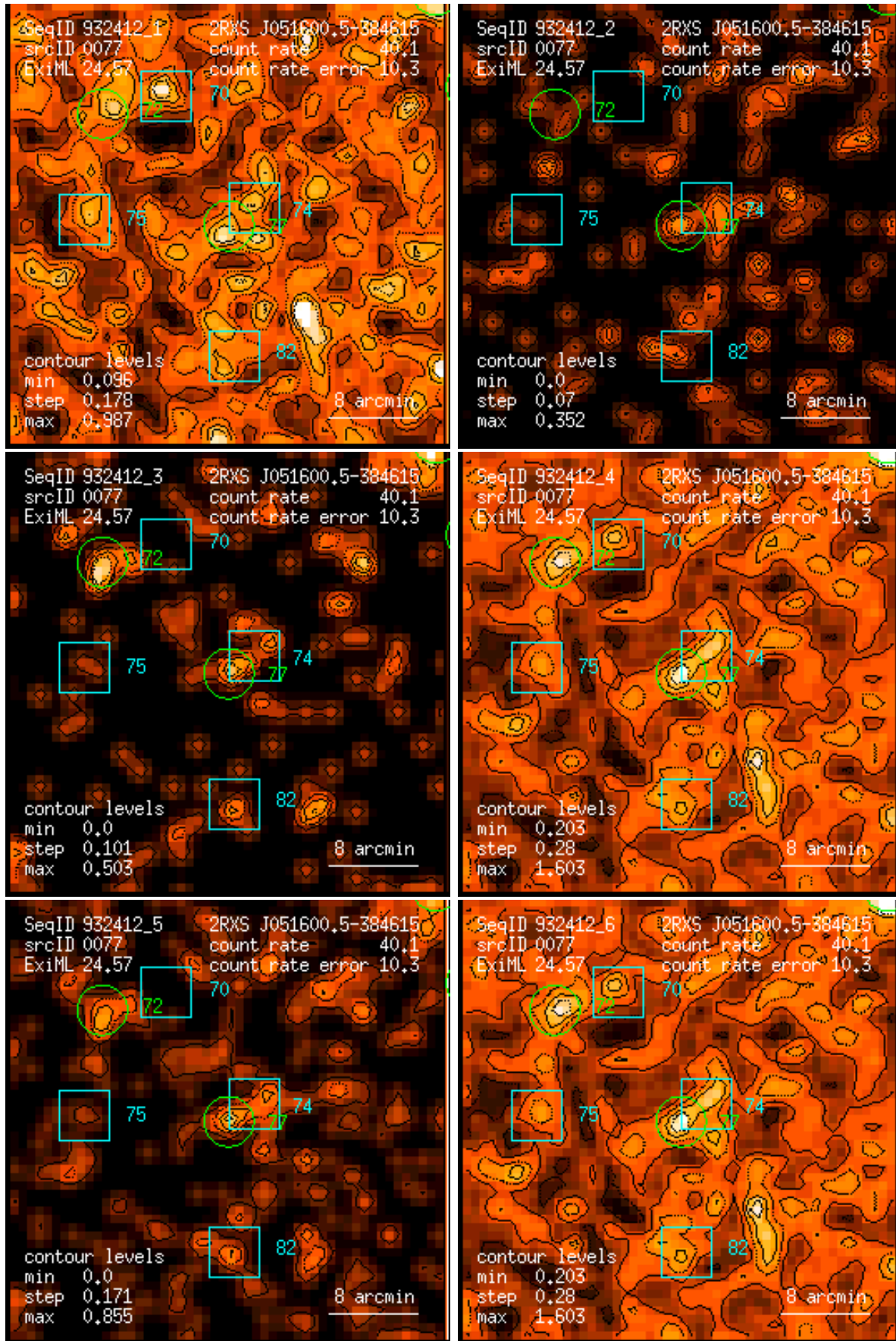
Figure 77: RASS 932412: detection 0077: band rate images, Gaussian filter: (1) PSPC channels 11 – 41, (2) 52 – 90, (3) 91 – 201, (4) 11 – 235, (5) 52 – 201, (6) 11 – 201. Broad band rates in counts/ks. Band rate contour levels in counts/ks/arcmin 2 .
