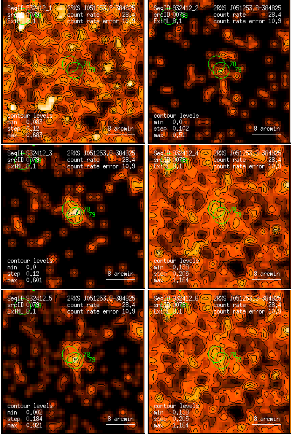
Figure 79: RASS 932412: detection 0079: band rate images, Gaussian filter: (1) PSPC channels 11 – 41, (2) 52 – 90, (3) 91 – 201, (4) 11 – 235, (5) 52 – 201, (6) 11 – 201. Broad band rates in counts/ks. Band rate contour levels in counts/ks/arcmin 2 .
