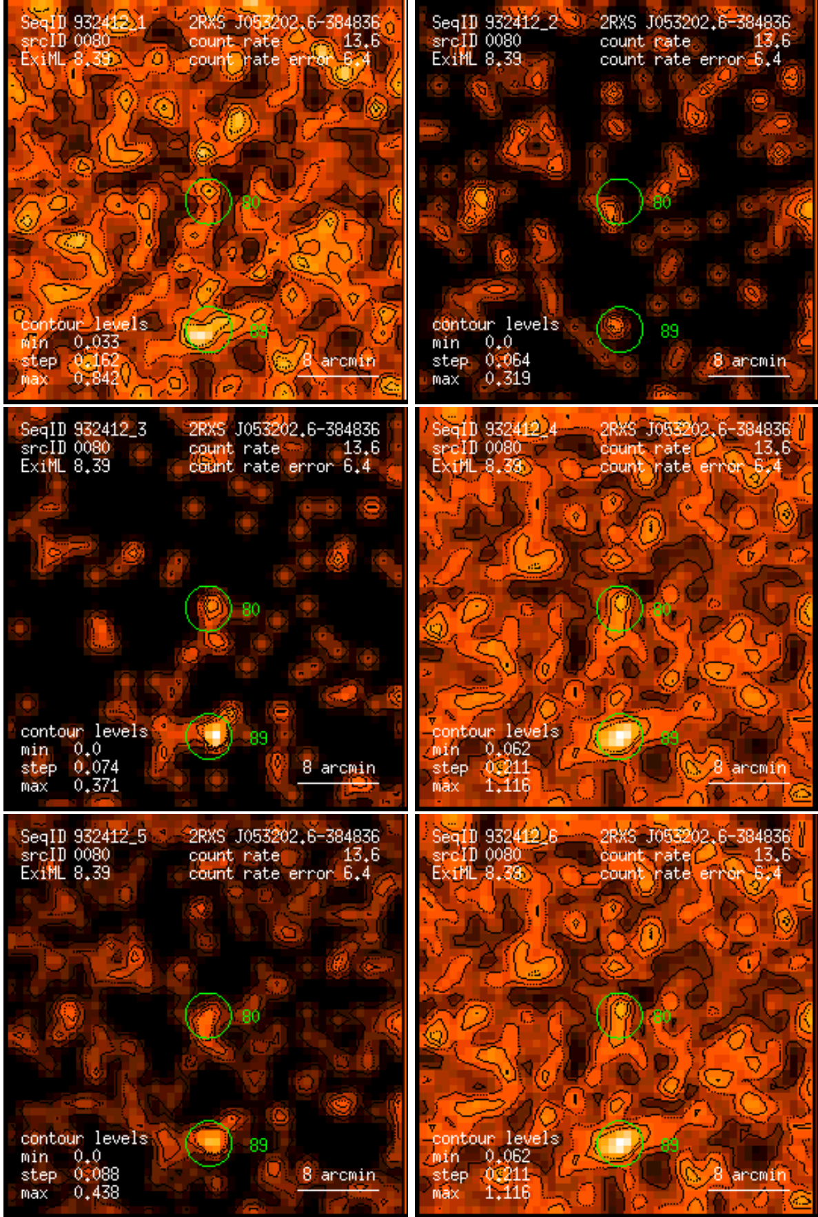
Figure 80: RASS 932412: detection 0080: band rate images, Gaussian filter: (1) PSPC channels 11 – 41, (2) 52 – 90, (3) 91 – 201, (4) 11 – 235, (5) 52 – 201, (6) 11 – 201. Broad band rates in counts/ks. Band rate contour levels in counts/ks/arcmin 2 .
