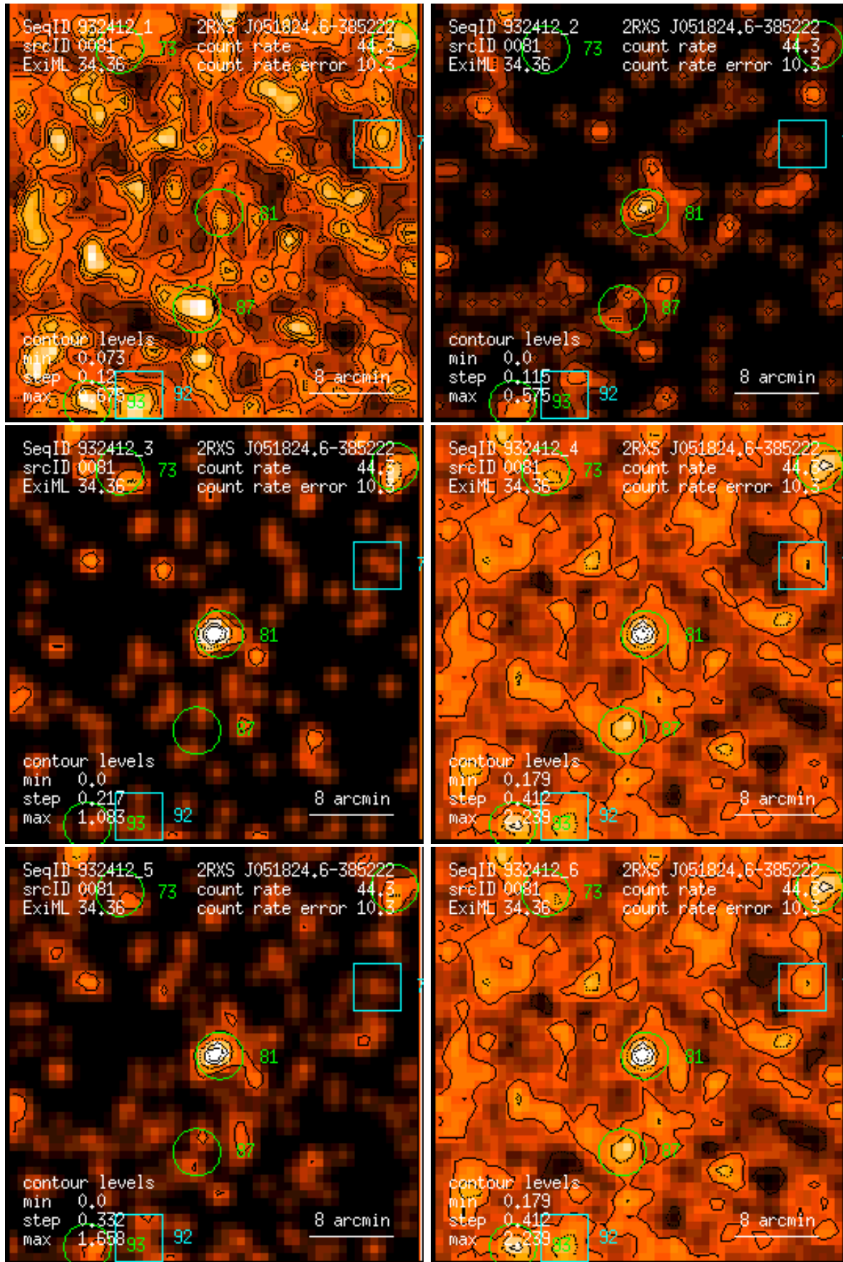
Figure 81: RASS 932412: detection 0081: band rate images, Gaussian filter: (1) PSPC channels 11 – 41, (2) 52 – 90, (3) 91 – 201, (4) 11 – 235, (5) 52 – 201, (6) 11 – 201. Broad band rates in counts/ks. Band rate contour levels in counts/ks/arcmin 2 .
