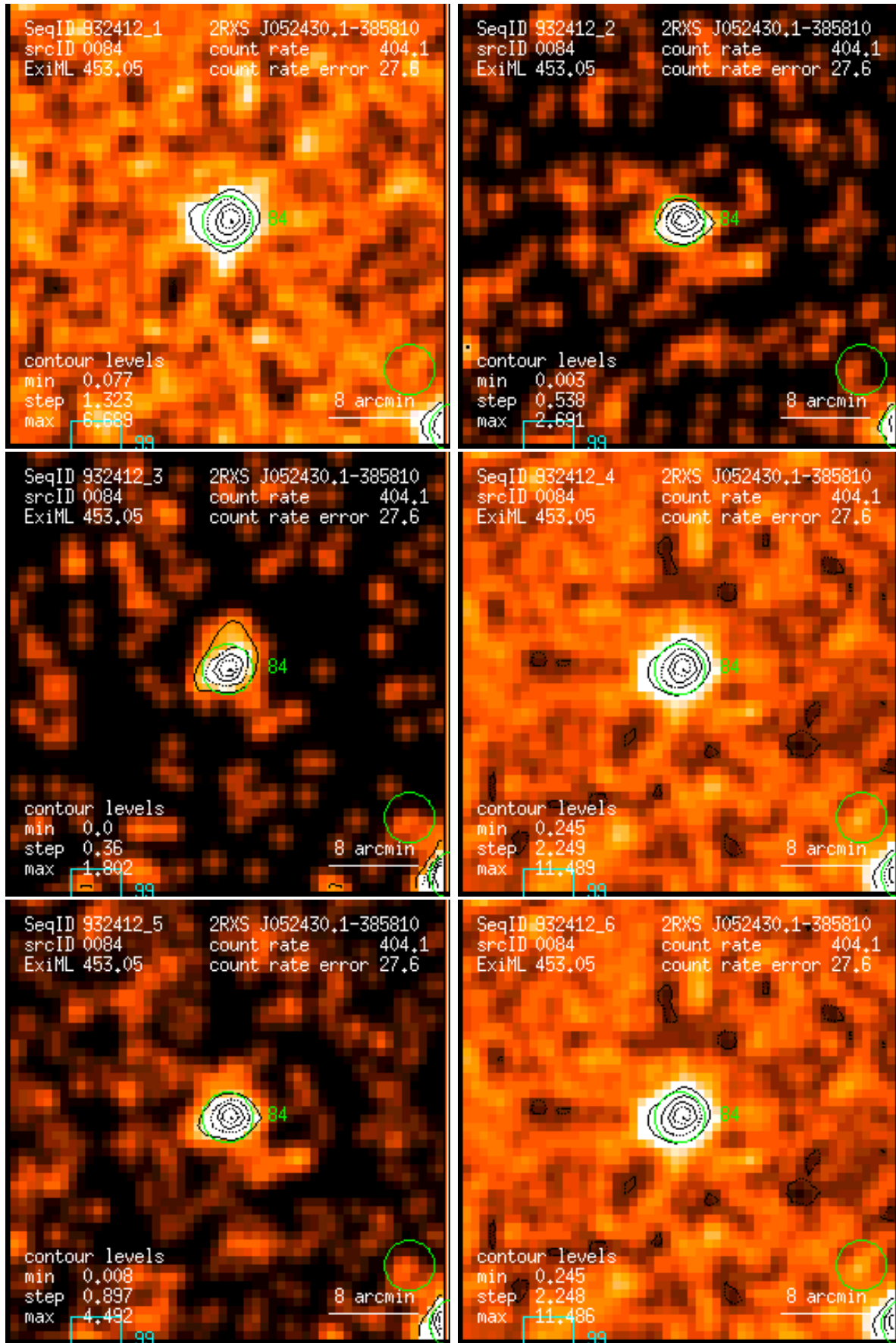
Figure 84: RASS 932412: detection 0084: band rate images, Gaussian filter: (1) PSPC channels 11 – 41, (2) 52 – 90, (3) 91 – 201, (4) 11 – 235, (5) 52 – 201, (6) 11 – 201. Broad band rates in counts/ks. Band rate contour levels in counts/ks/arcmin 2 .
