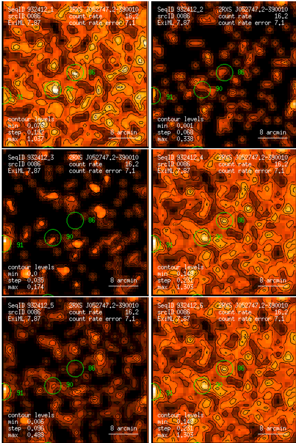
Figure 86: RASS 932412: detection 0086: band rate images, Gaussian filter: (1) PSPC channels 11 – 41, (2) 52 – 90, (3) 91 – 201, (4) 11 – 235, (5) 52 – 201, (6) 11 – 201. Broad band rates in counts/ks. Band rate contour levels in counts/ks/arcmin 2 .
