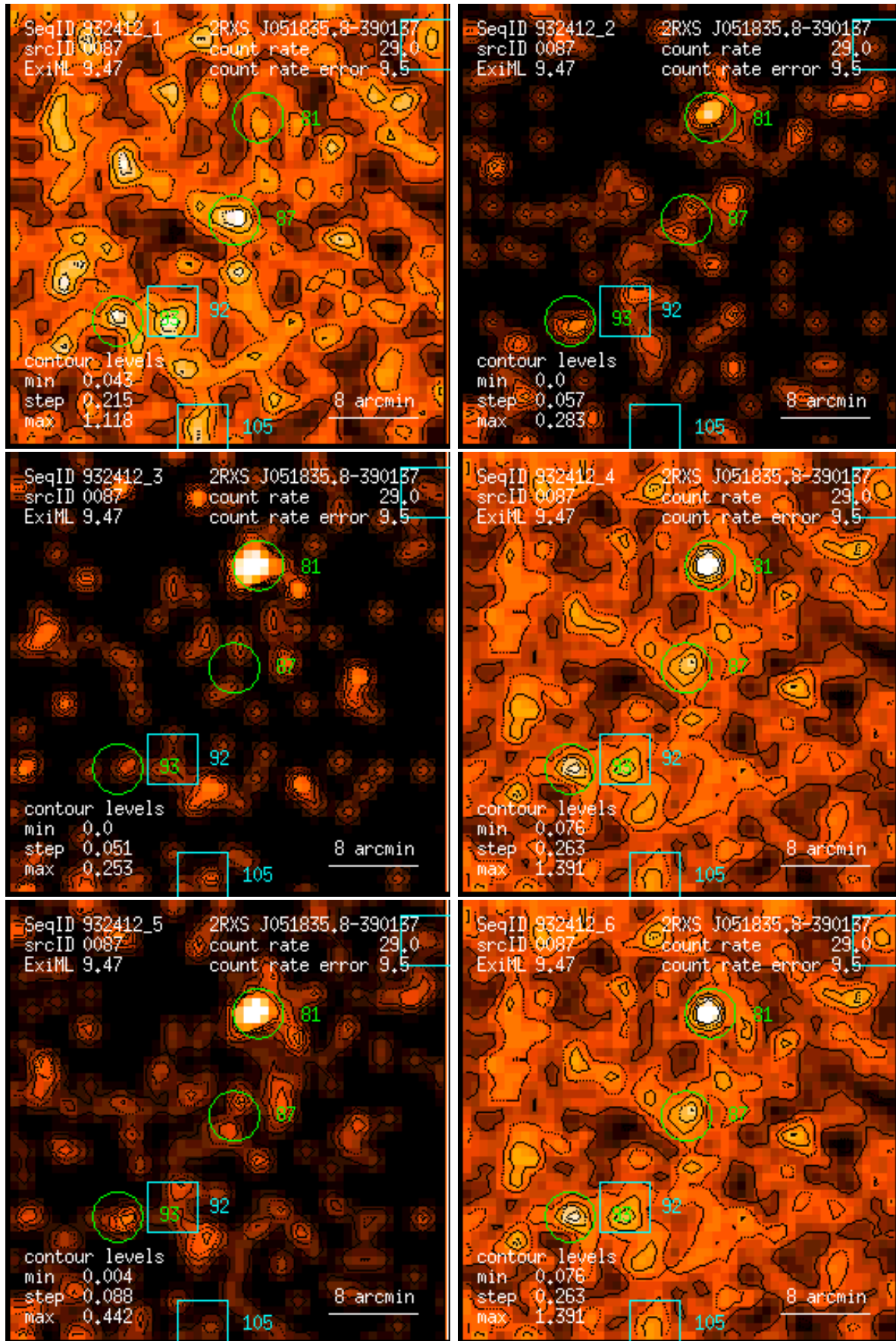
Figure 87: RASS 932412: detection 0087: band rate images, Gaussian filter: (1) PSPC channels 11 – 41, (2) 52 – 90, (3) 91 – 201, (4) 11 – 235, (5) 52 – 201, (6) 11 – 201. Broad band rates in counts/ks. Band rate contour levels in counts/ks/arcmin 2 .
