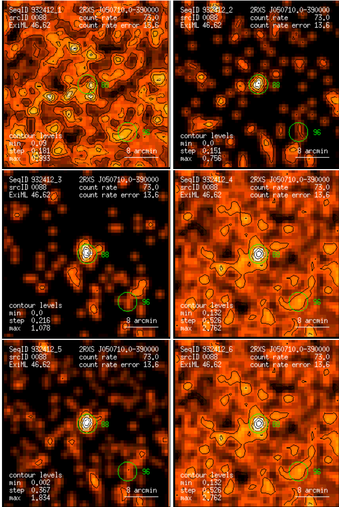
Figure 88: RASS 932412: detection 0088: band rate images, Gaussian filter: (1) PSPC channels 11 – 41, (2) 52 – 90, (3) 91 – 201, (4) 11 – 235, (5) 52 – 201, (6) 11 – 201. Broad band rates in counts/ks. Band rate contour levels in counts/ks/arcmin 2 .
