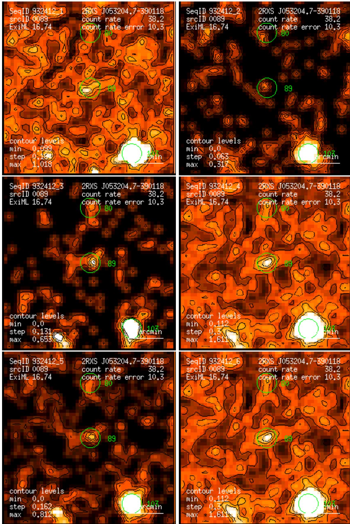
Figure 89: RASS 932412: detection 0089: band rate images, Gaussian filter: (1) PSPC channels 11 – 41, (2) 52 – 90, (3) 91 – 201, (4) 11 – 235, (5) 52 – 201, (6) 11 – 201. Broad band rates in counts/ks. Band rate contour levels in counts/ks/arcmin 2 .
