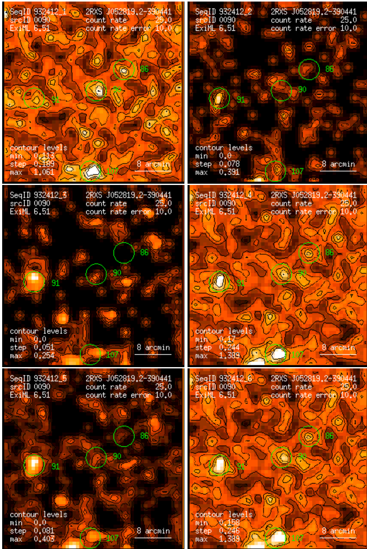
Figure 90: RASS 932412: detection 0090: band rate images, Gaussian filter: (1) PSPC channels 11 – 41, (2) 52 – 90, (3) 91 – 201, (4) 11 – 235, (5) 52 – 201, (6) 11 – 201. Broad band rates in counts/ks. Band rate contour levels in counts/ks/arcmin 2 .
