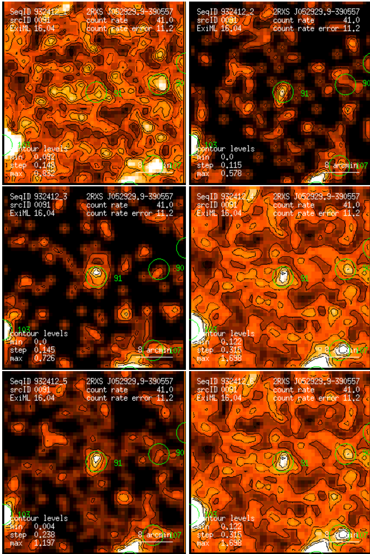
Figure 91: RASS 932412: detection 0091: band rate images, Gaussian filter: (1) PSPC channels 11 – 41, (2) 52 – 90, (3) 91 – 201, (4) 11 – 235, (5) 52 – 201, (6) 11 – 201. Broad band rates in counts/ks. Band rate contour levels in counts/ks/arcmin 2 .
