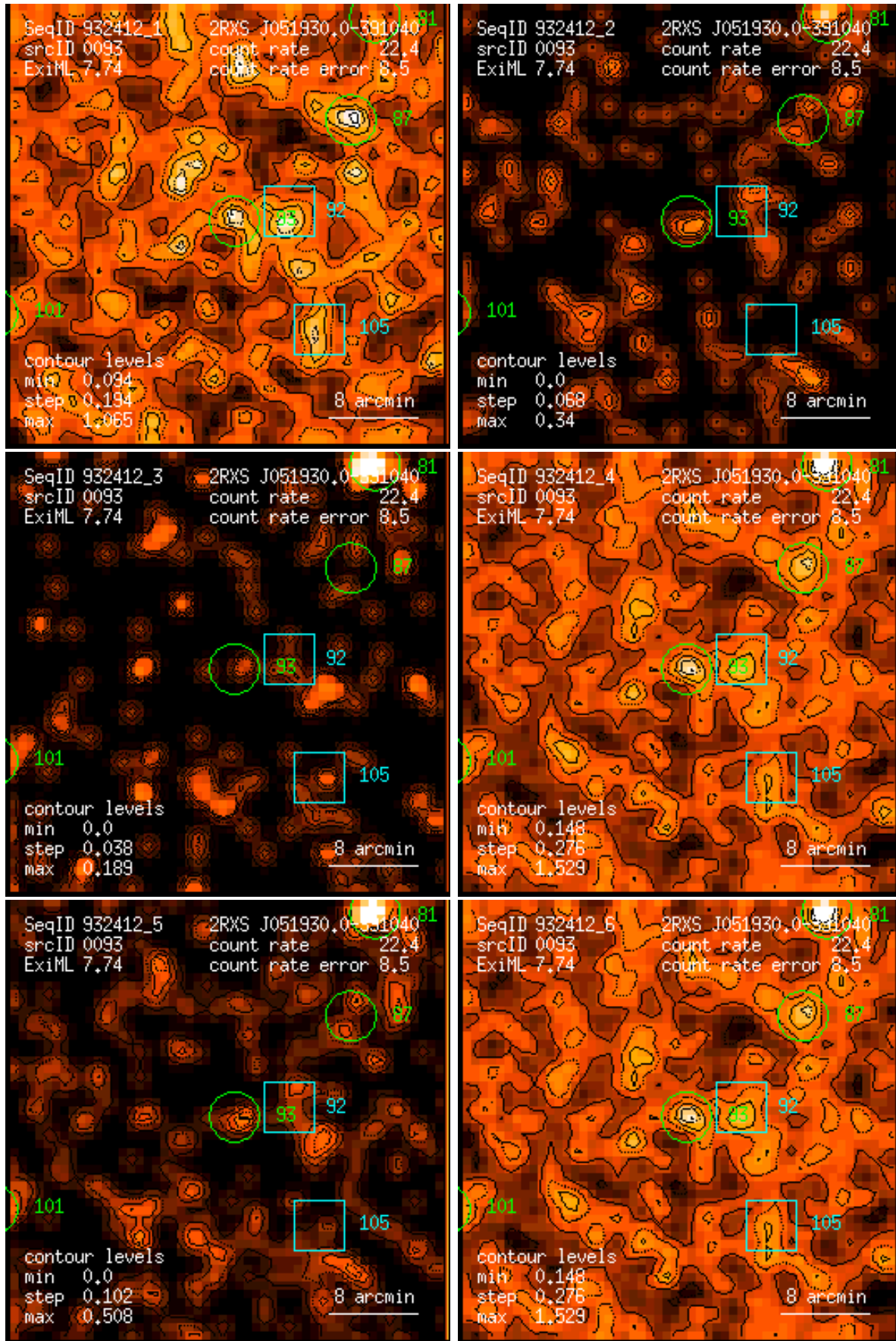
Figure 93: RASS 932412: detection 0093: band rate images, Gaussian filter: (1) PSPC channels 11 – 41, (2) 52 – 90, (3) 91 – 201, (4) 11 – 235, (5) 52 – 201, (6) 11 – 201. Broad band rates in counts/ks. Band rate contour levels in counts/ks/arcmin 2 .
