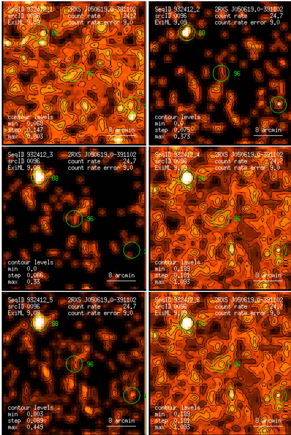
Figure 96: RASS 932412: detection 0096: band rate images, Gaussian filter: (1) PSPC channels 11 – 41, (2) 52 – 90, (3) 91 – 201, (4) 11 – 235, (5) 52 – 201, (6) 11 – 201. Broad band rates in counts/ks. Band rate contour levels in counts/ks/arcmin 2 .
