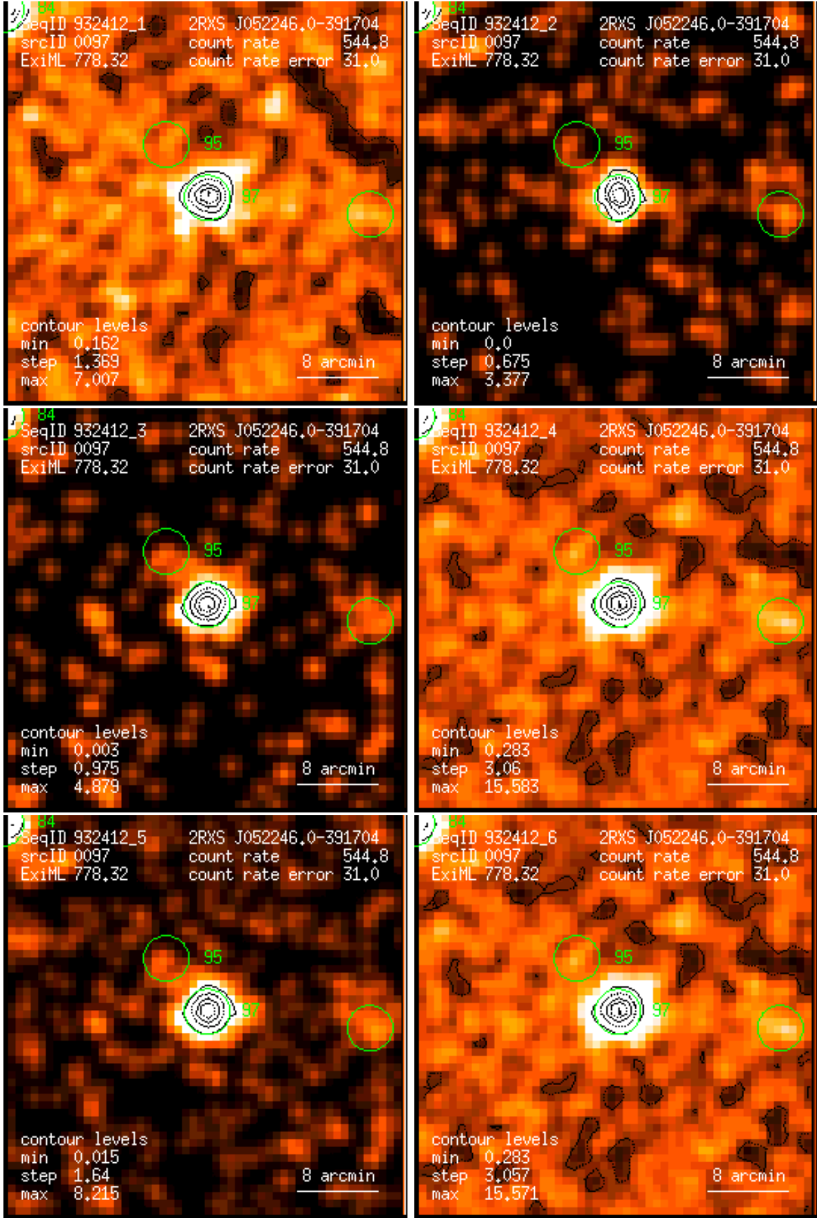
Figure 97: RASS 932412: detection 0097: band rate images, Gaussian filter: (1) PSPC channels 11 – 41, (2) 52 – 90, (3) 91 – 201, (4) 11 – 235, (5) 52 – 201, (6) 11 – 201. Broad band rates in counts/ks. Band rate contour levels in counts/ks/arcmin 2 .
