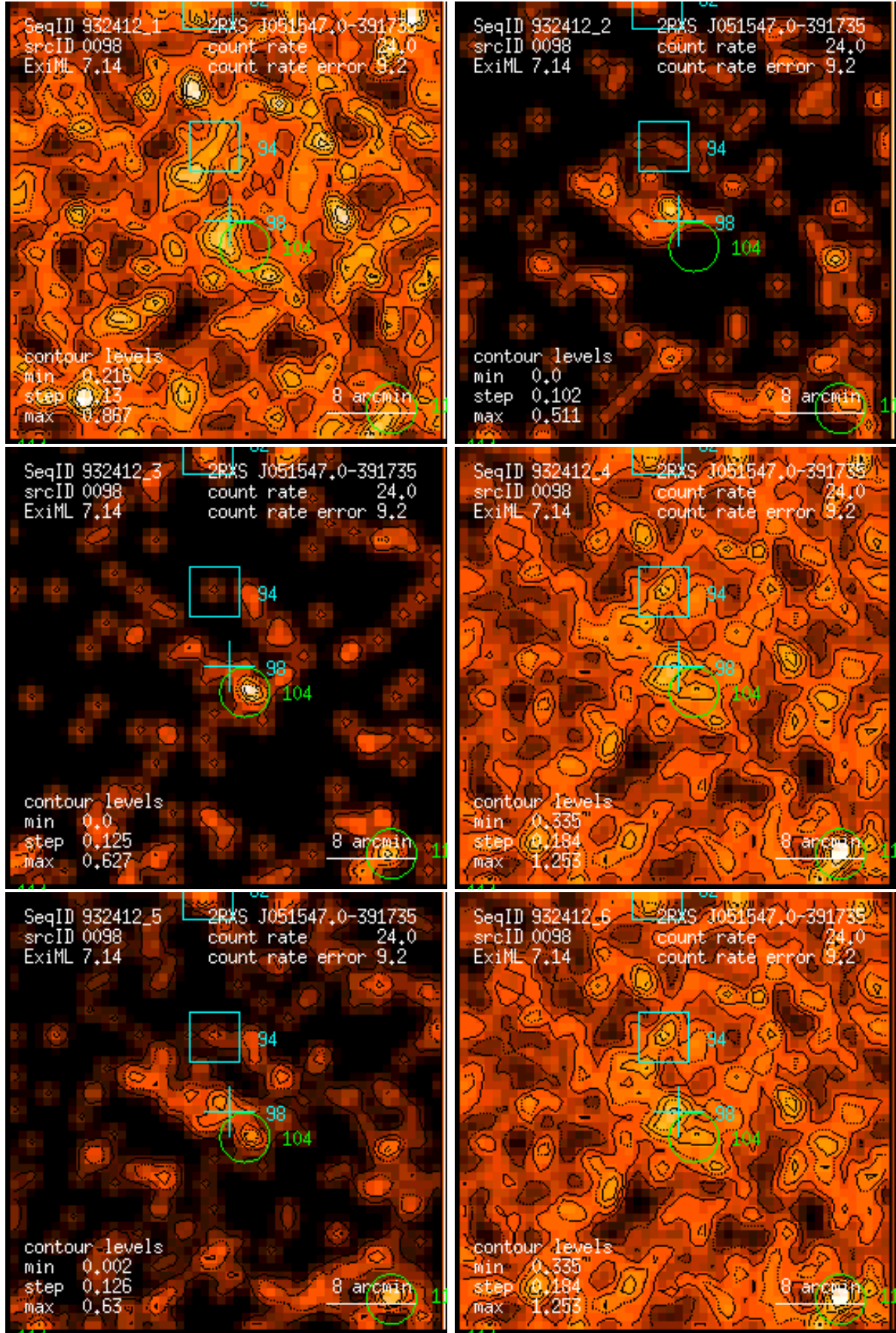
Figure 98: RASS 932412: detection 0098: band rate images, Gaussian filter: (1) PSPC channels 11 – 41, (2) 52 – 90, (3) 91 – 201, (4) 11 – 235, (5) 52 – 201, (6) 11 – 201. Broad band rates in counts/ks. Band rate contour levels in counts/ks/arcmin 2 .
