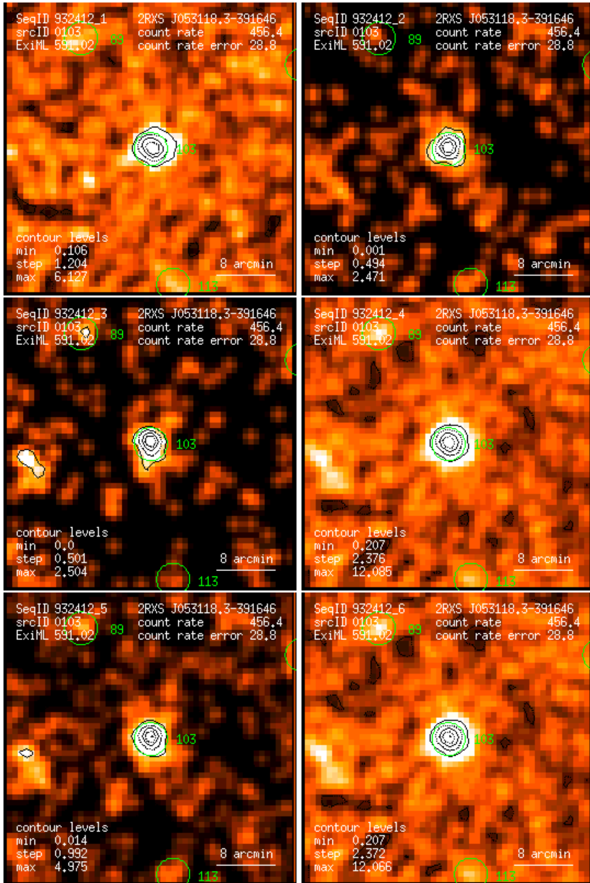
Figure 103: RASS 932412: detection 0103: band rate images, Gaussian filter: (1) PSPC channels 11 – 41, (2) 52 – 90, (3) 91 – 201, (4) 11 – 235, (5) 52 – 201, (6) 11 – 201. Broad band rates in counts/ks. Band rate contour levels in counts/ks/arcmin 2 .
