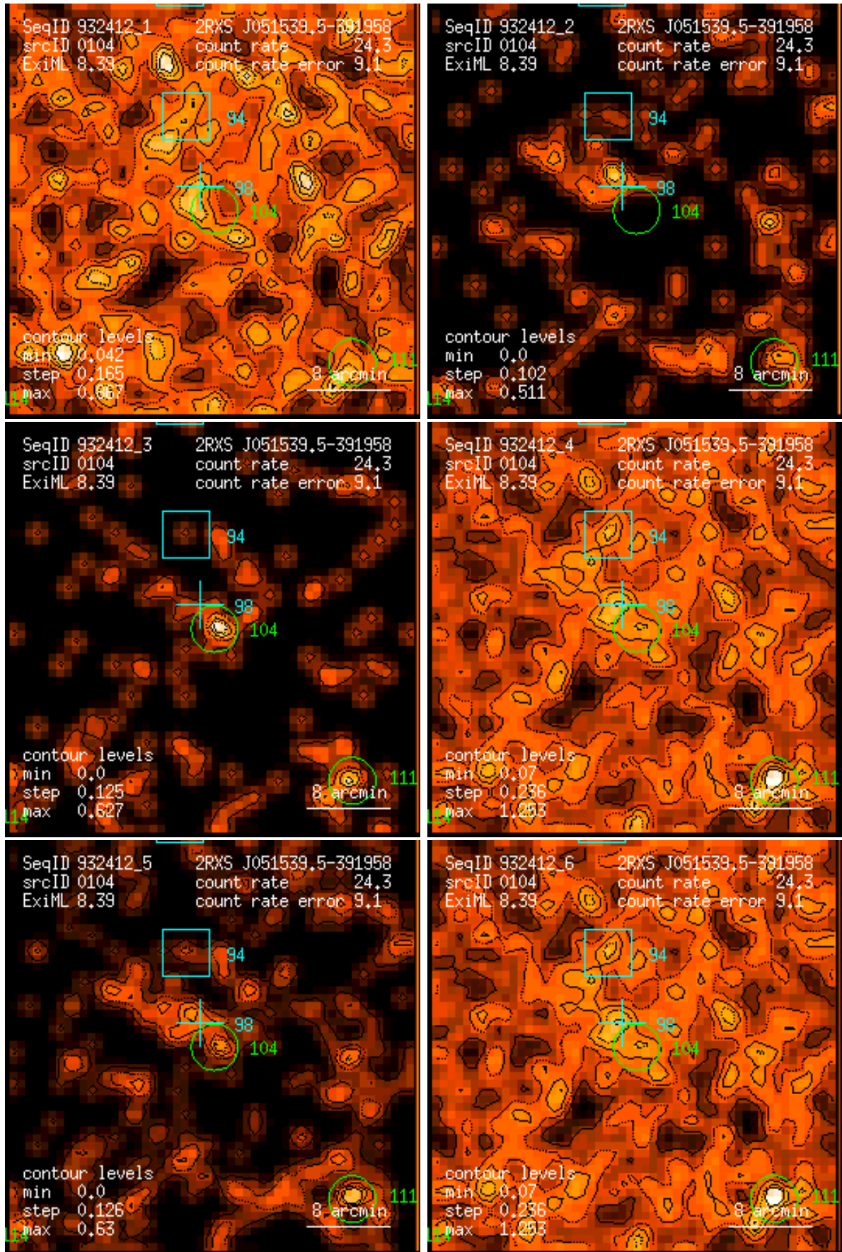
Figure 104: RASS 932412: detection 0104: band rate images, Gaussian filter: (1) PSPC channels 11 – 41, (2) 52 – 90, (3) 91 – 201, (4) 11 – 235, (5) 52 – 201, (6) 11 – 201. Broad band rates in counts/ks. Band rate contour levels in counts/ks/arcmin 2 .
