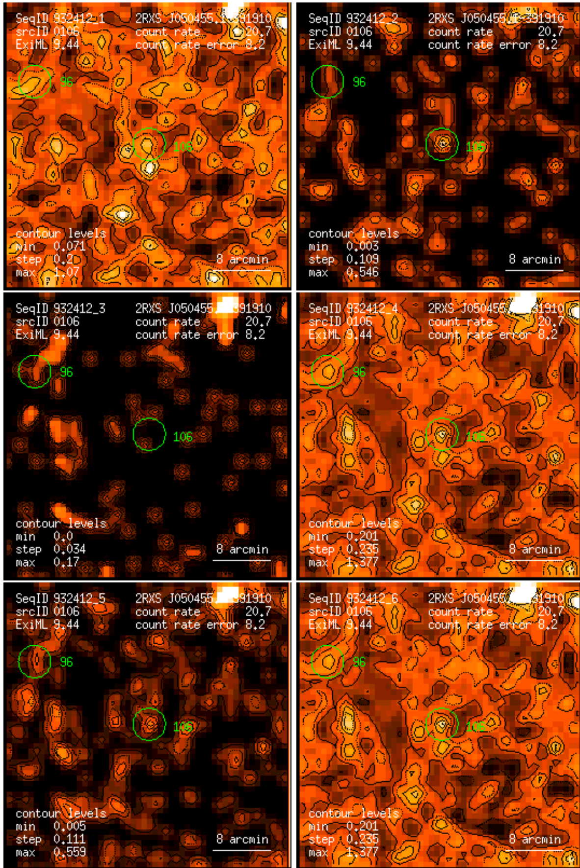
Figure 106: RASS 932412: detection 0106: band rate images, Gaussian filter: (1) PSPC channels 11 – 41, (2) 52 – 90, (3) 91 – 201, (4) 11 – 235, (5) 52 – 201, (6) 11 – 201. Broad band rates in counts/ks. Band rate contour levels in counts/ks/arcmin 2 .
