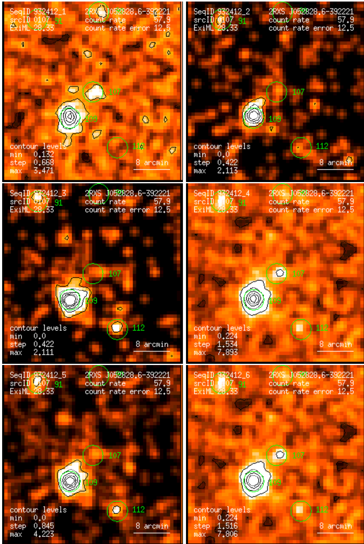
Figure 107: RASS 932412: detection 0107: band rate images, Gaussian filter: (1) PSPC channels 11 – 41, (2) 52 – 90, (3) 91 – 201, (4) 11 – 235, (5) 52 – 201, (6) 11 – 201. Broad band rates in counts/ks. Band rate contour levels in counts/ks/arcmin 2 .
