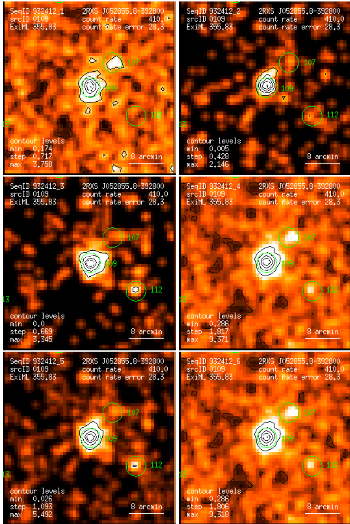
Figure 109: RASS 932412: detection 0109: band rate images, Gaussian filter: (1) PSPC channels 11 – 41, (2) 52 – 90, (3) 91 – 201, (4) 11 – 235, (5) 52 – 201, (6) 11 – 201. Broad band rates in counts/ks. Band rate contour levels in counts/ks/arcmin 2 .
