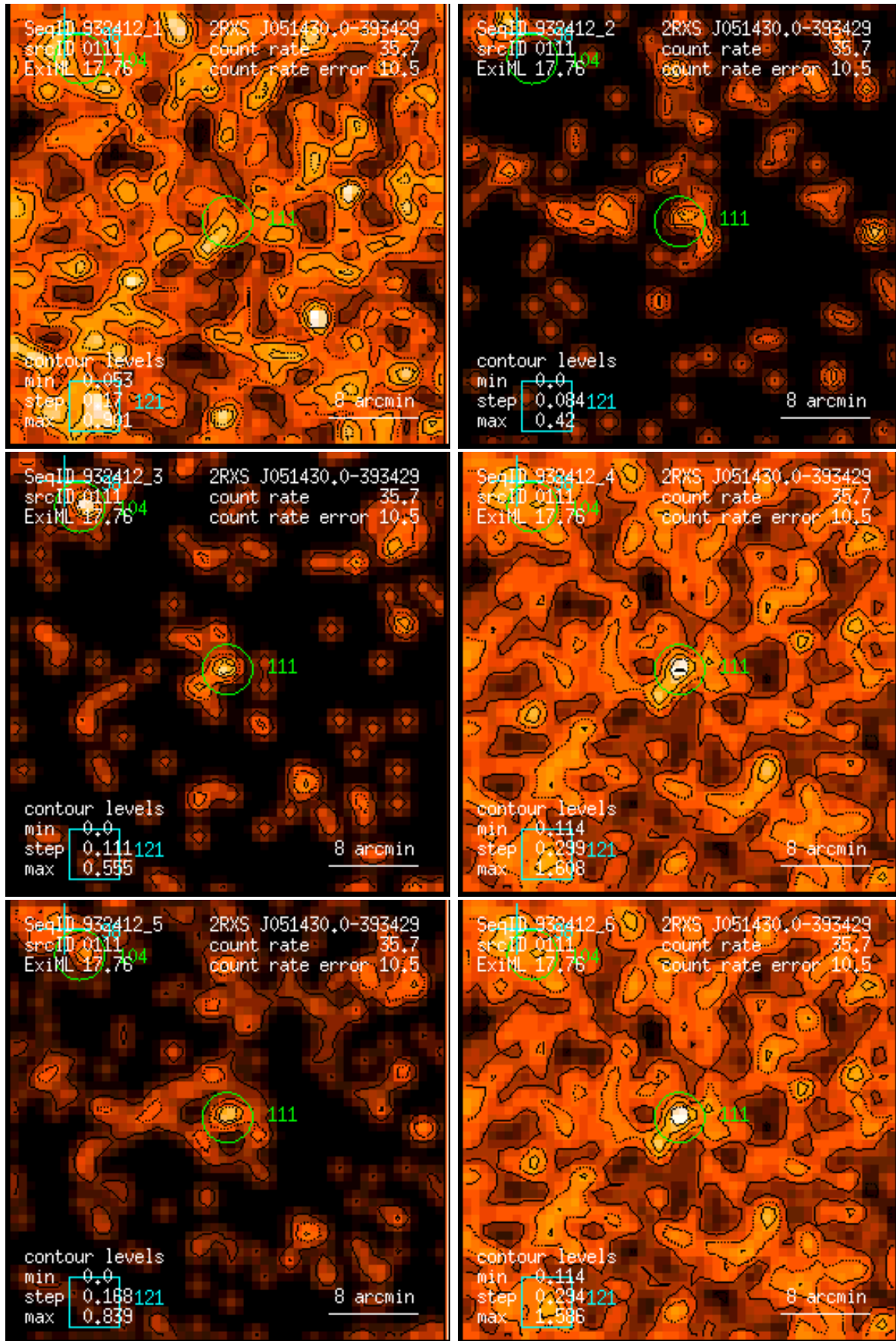
Figure 111: RASS 932412: detection 0111: band rate images, Gaussian filter: (1) PSPC channels 11 – 41, (2) 52 – 90, (3) 91 – 201, (4) 11 – 235, (5) 52 – 201, (6) 11 – 201. Broad band rates in counts/ks. Band rate contour levels in counts/ks/arcmin 2 .
