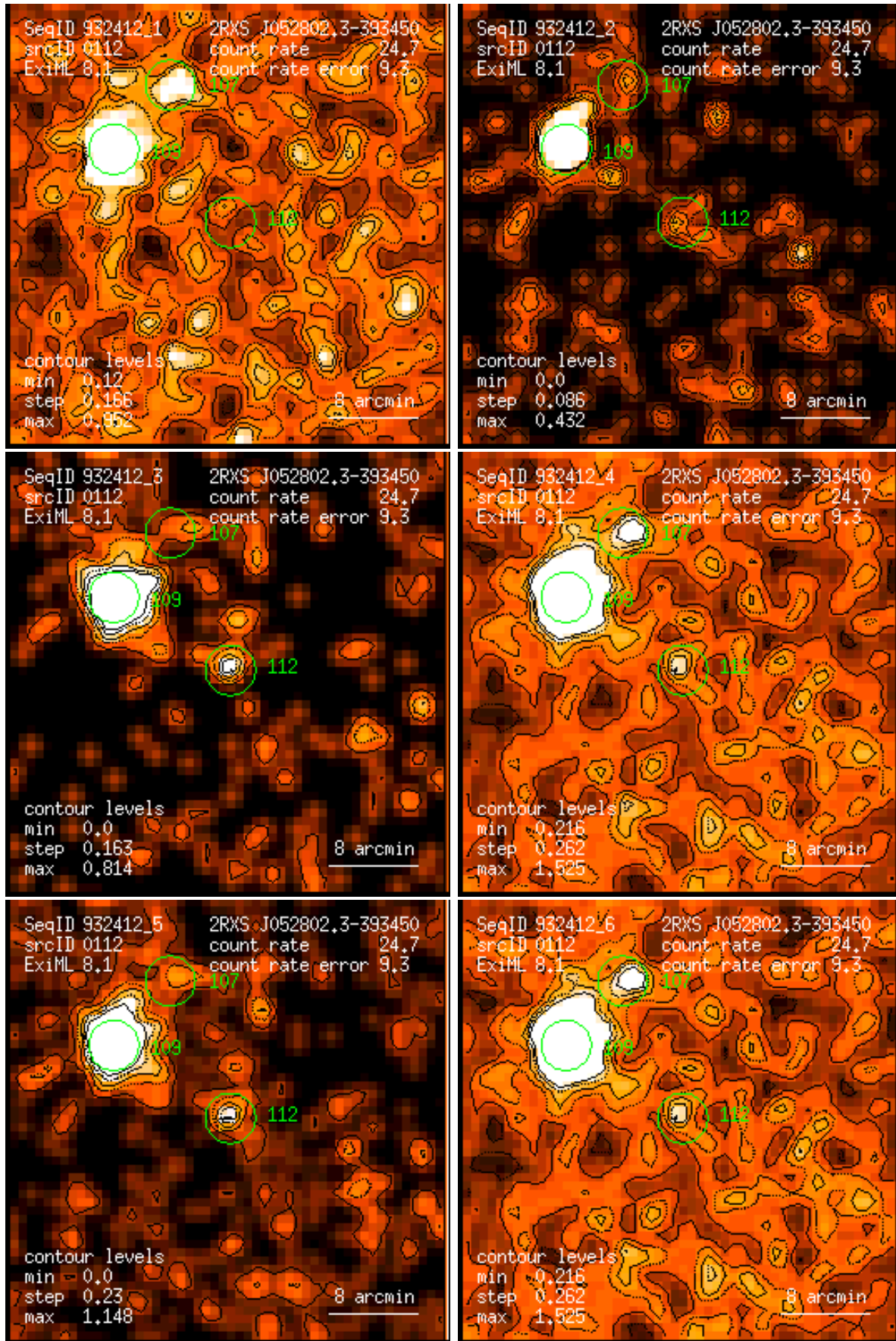
Figure 112: RASS 932412: detection 0112: band rate images, Gaussian filter: (1) PSPC channels 11 – 41, (2) 52 – 90, (3) 91 – 201, (4) 11 – 235, (5) 52 – 201, (6) 11 – 201. Broad band rates in counts/ks. Band rate contour levels in counts/ks/arcmin 2 .
