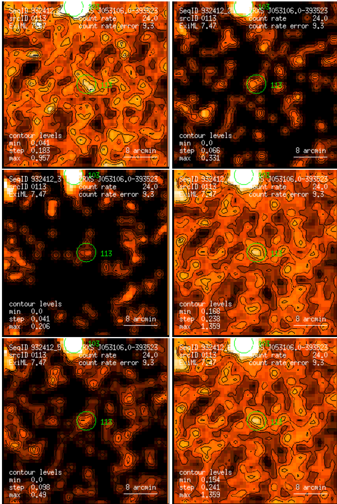
Figure 113: RASS 932412: detection 0113: band rate images, Gaussian filter: (1) PSPC channels 11 – 41, (2) 52 – 90, (3) 91 – 201, (4) 11 – 235, (5) 52 – 201, (6) 11 – 201. Broad band rates in counts/ks. Band rate contour levels in counts/ks/arcmin 2 .
