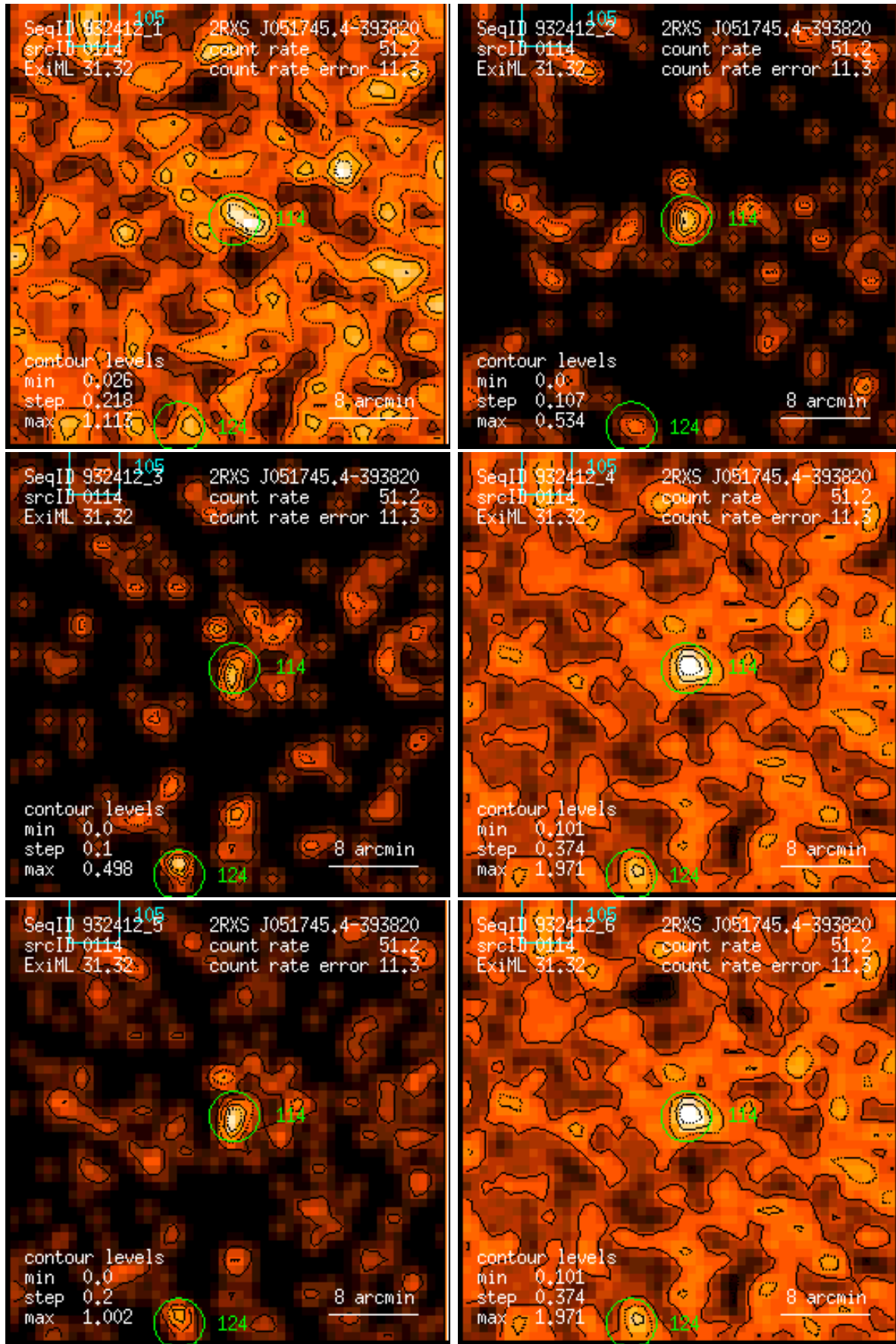
Figure 114: RASS 932412: detection 0114: band rate images, Gaussian filter: (1) PSPC channels 11 – 41, (2) 52 – 90, (3) 91 – 201, (4) 11 – 235, (5) 52 – 201, (6) 11 – 201. Broad band rates in counts/ks. Band rate contour levels in counts/ks/arcmin 2 .
