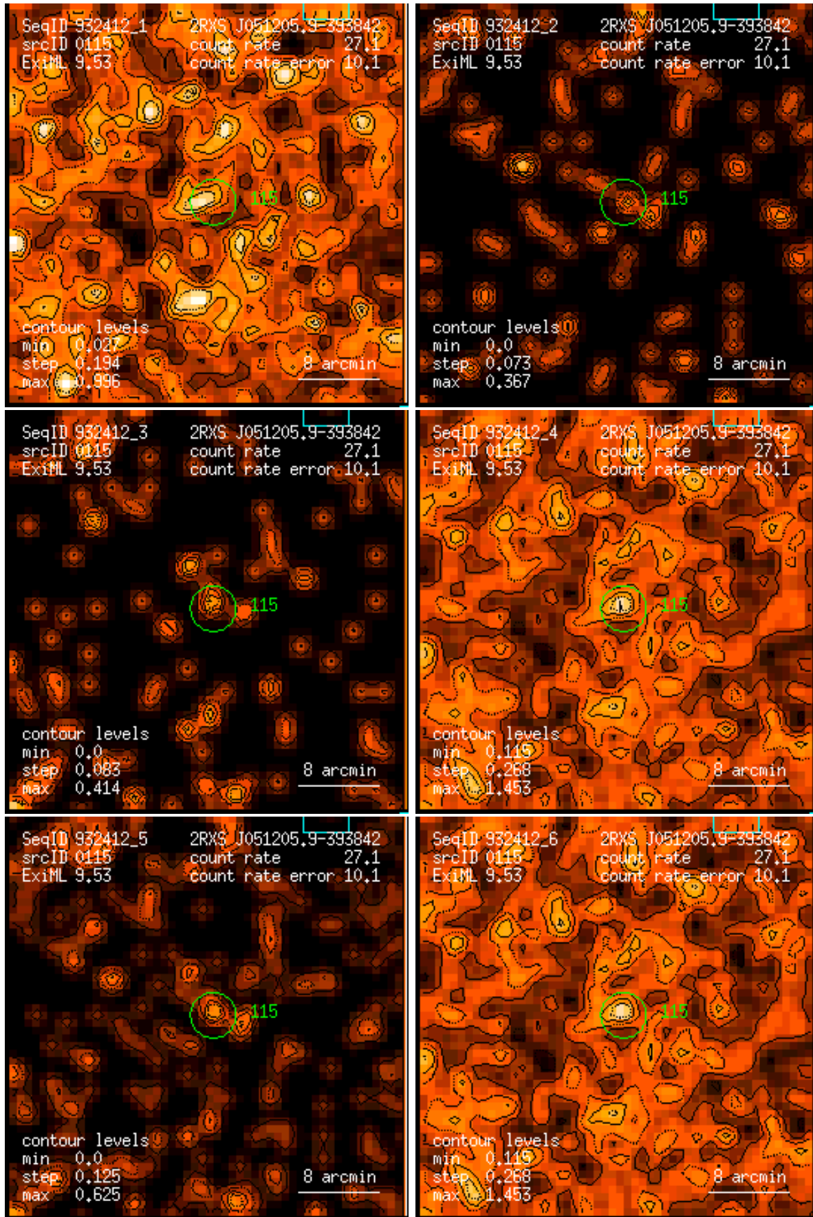
Figure 115: RASS 932412: detection 0115: band rate images, Gaussian filter: (1) PSPC channels 11 – 41, (2) 52 – 90, (3) 91 – 201, (4) 11 – 235, (5) 52 – 201, (6) 11 – 201. Broad band rates in counts/ks. Band rate contour levels in counts/ks/arcmin 2 .
