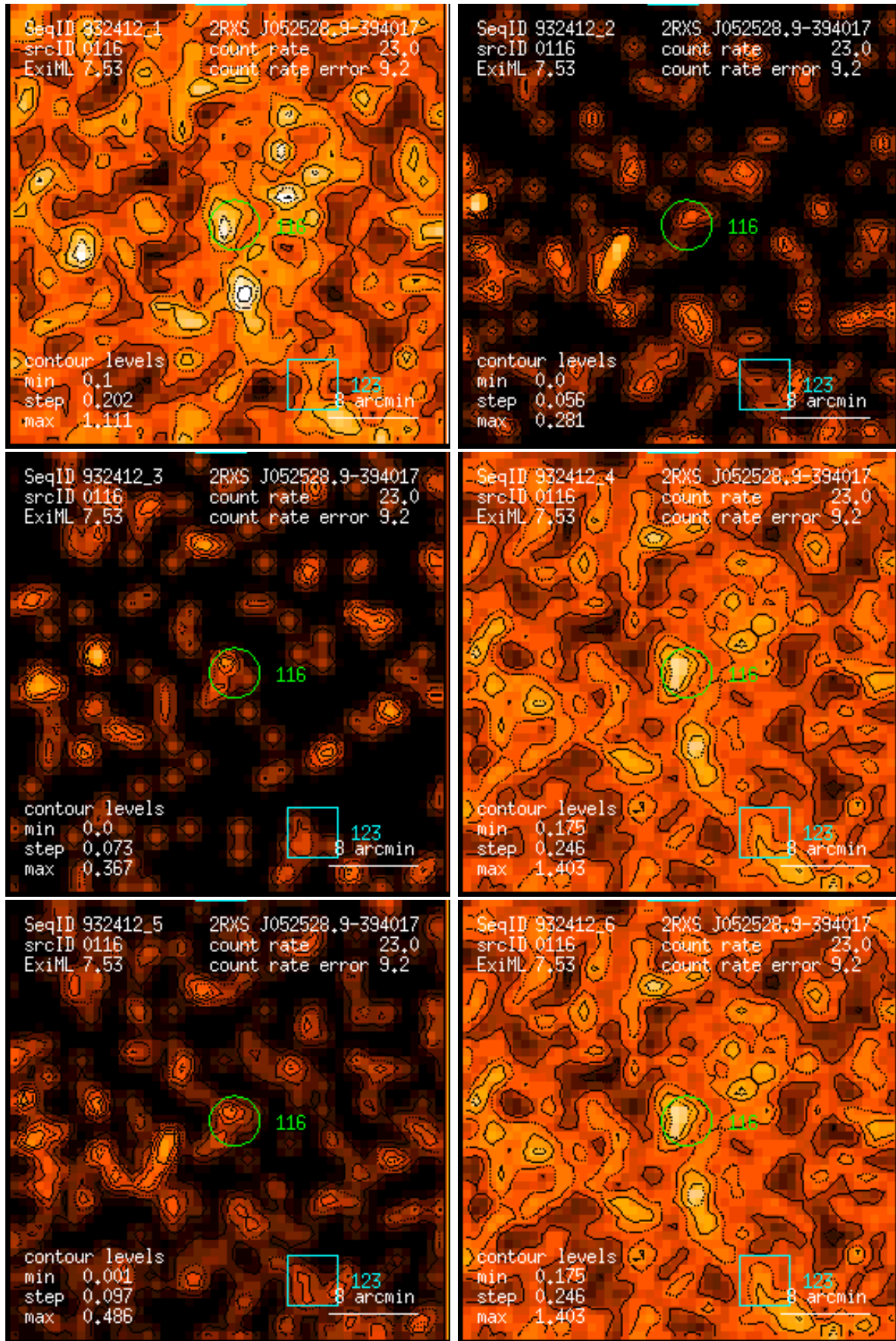
Figure 116: RASS 932412: detection 0116: band rate images, Gaussian filter: (1) PSPC channels 11 – 41, (2) 52 – 90, (3) 91 – 201, (4) 11 – 235, (5) 52 – 201, (6) 11 – 201. Broad band rates in counts/ks. Band rate contour levels in counts/ks/arcmin 2 .
