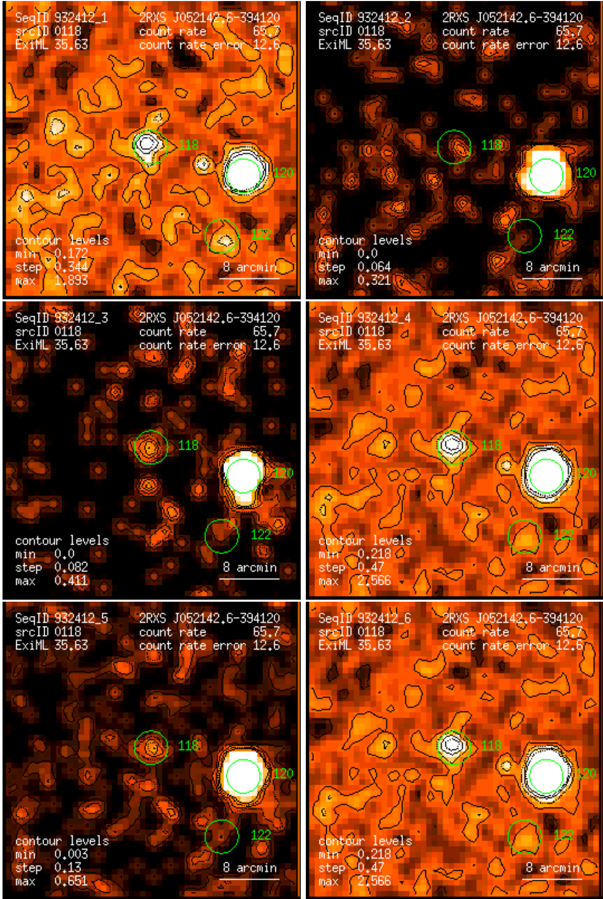
Figure 118: RASS 932412: detection 0118: band rate images, Gaussian filter: (1) PSPC channels 11 – 41, (2) 52 – 90, (3) 91 – 201, (4) 11 – 235, (5) 52 – 201, (6) 11 – 201. Broad band rates in counts/ks. Band rate contour levels in counts/ks/arcmin 2 .
