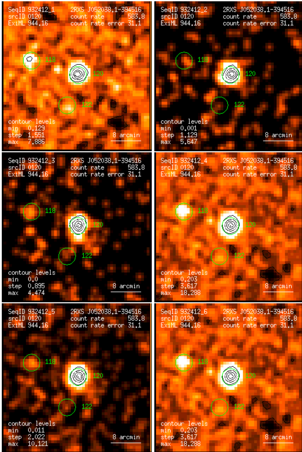
Figure 120: RASS 932412: detection 0120: band rate images, Gaussian filter: (1) PSPC channels 11 – 41, (2) 52 – 90, (3) 91 – 201, (4) 11 – 235, (5) 52 – 201, (6) 11 – 201. Broad band rates in counts/ks. Band rate contour levels in counts/ks/arcmin 2 .
