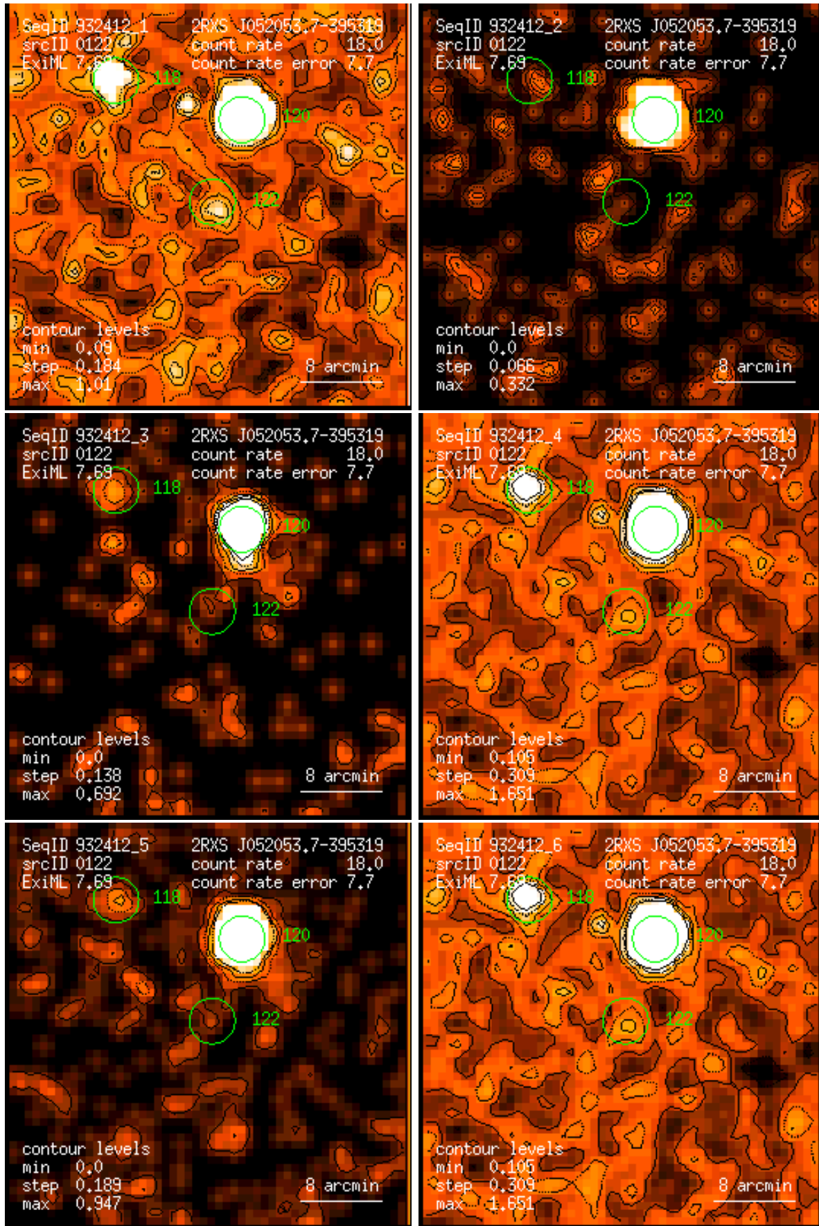
Figure 122: RASS 932412: detection 0122: band rate images, Gaussian filter: (1) PSPC channels 11 – 41, (2) 52 – 90, (3) 91 – 201, (4) 11 – 235, (5) 52 – 201, (6) 11 – 201. Broad band rates in counts/ks. Band rate contour levels in counts/ks/arcmin 2 .
