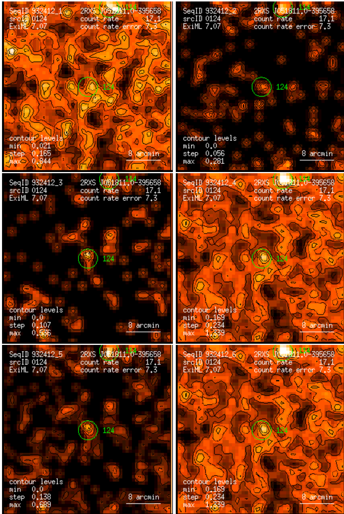
Figure 124: RASS 932412: detection 0124: band rate images, Gaussian filter: (1) PSPC channels 11 – 41, (2) 52 – 90, (3) 91 – 201, (4) 11 – 235, (5) 52 – 201, (6) 11 – 201. Broad band rates in counts/ks. Band rate contour levels in counts/ks/arcmin 2 .
