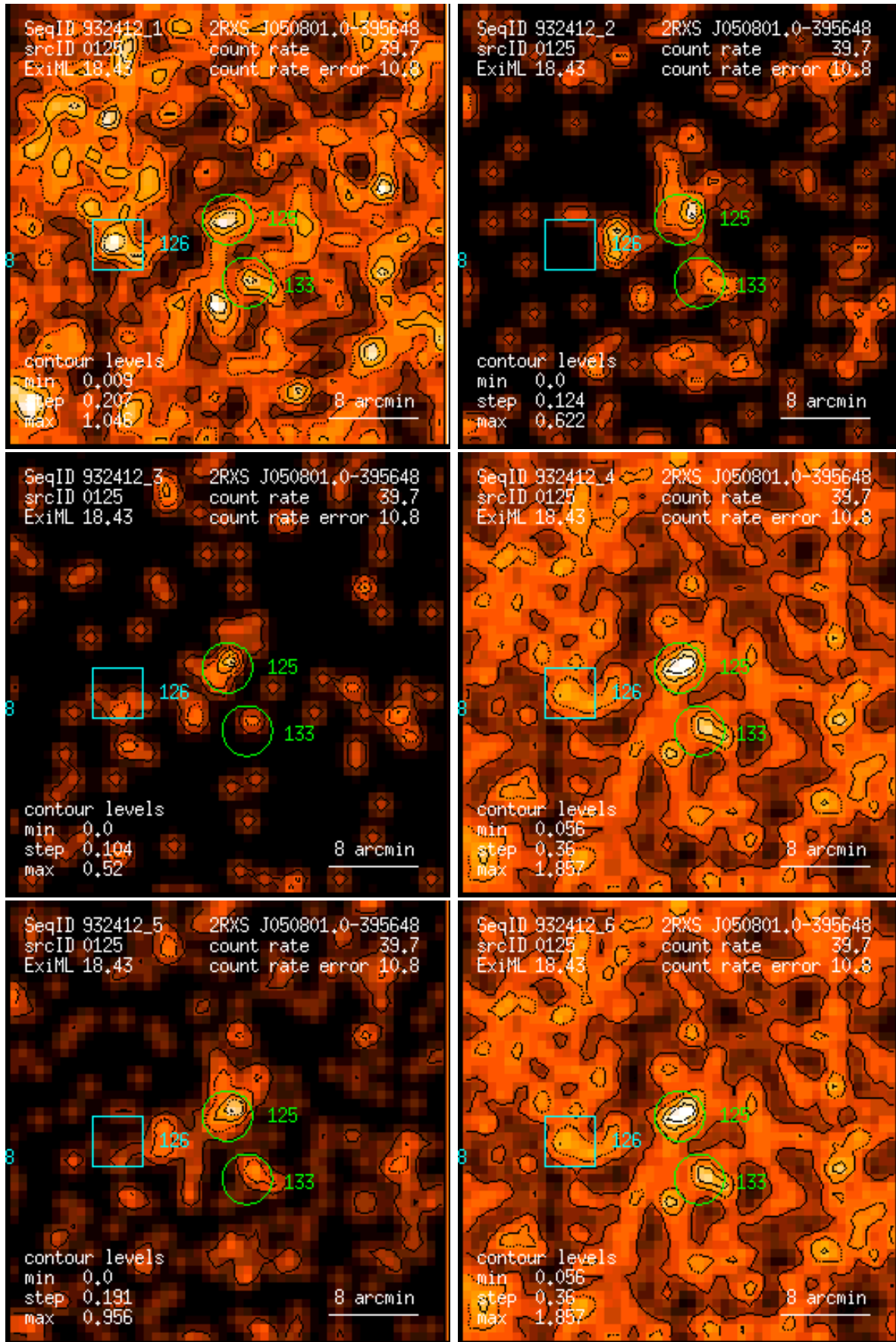
Figure 125: RASS 932412: detection 0125: band rate images, Gaussian filter: (1) PSPC channels 11 – 41, (2) 52 – 90, (3) 91 – 201, (4) 11 – 235, (5) 52 – 201, (6) 11 – 201. Broad band rates in counts/ks. Band rate contour levels in counts/ks/arcmin 2 .
