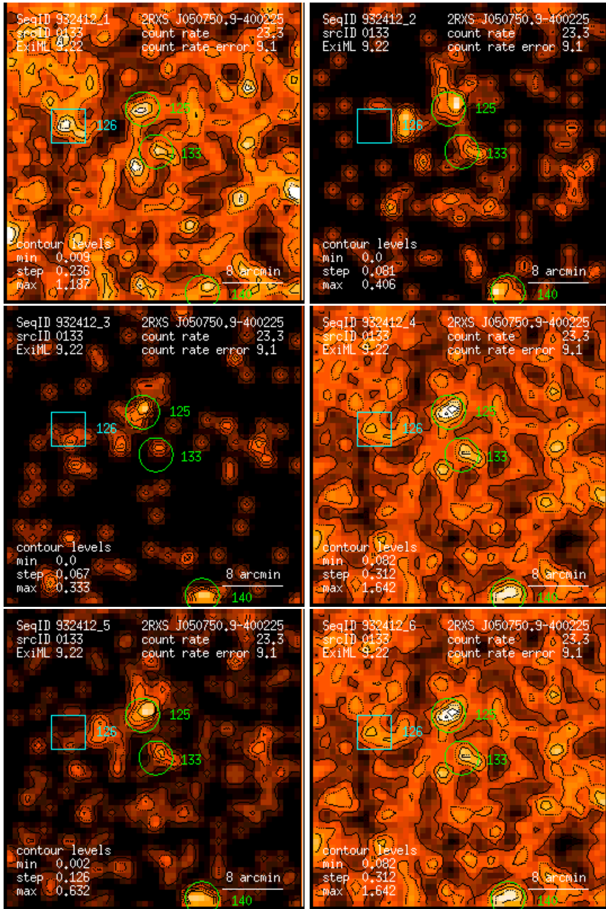
Figure 133: RASS 932412: detection 0133: band rate images, Gaussian filter: (1) PSPC channels 11 – 41, (2) 52 – 90, (3) 91 – 201, (4) 11 – 235, (5) 52 – 201, (6) 11 – 201. Broad band rates in counts/ks. Band rate contour levels in counts/ks/arcmin 2 .
