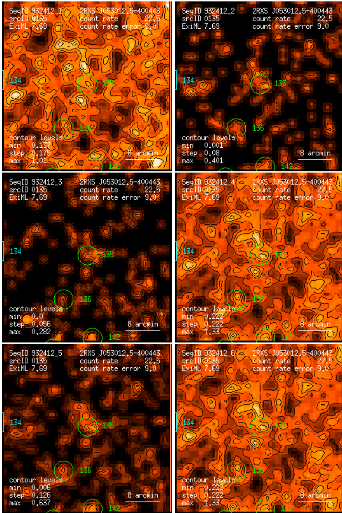
Figure 135: RASS 932412: detection 0135: band rate images, Gaussian filter: (1) PSPC channels 11 – 41, (2) 52 – 90, (3) 91 – 201, (4) 11 – 235, (5) 52 – 201, (6) 11 – 201. Broad band rates in counts/ks. Band rate contour levels in counts/ks/arcmin 2 .
