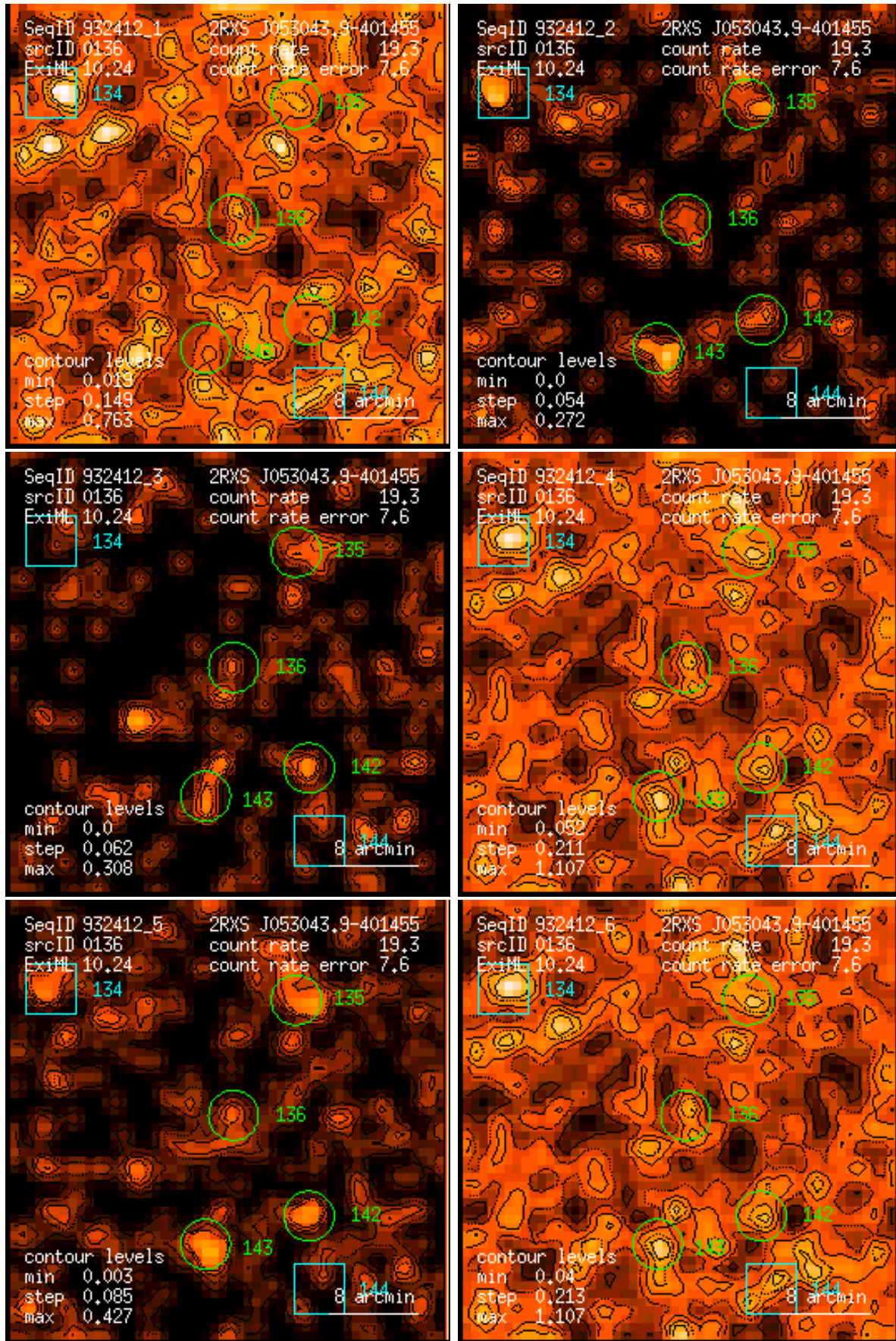
Figure 136: RASS 932412: detection 0136: band rate images, Gaussian filter: (1) PSPC channels 11 – 41, (2) 52 – 90, (3) 91 – 201, (4) 11 – 235, (5) 52 – 201, (6) 11 – 201. Broad band rates in counts/ks. Band rate contour levels in counts/ks/arcmin 2 .
