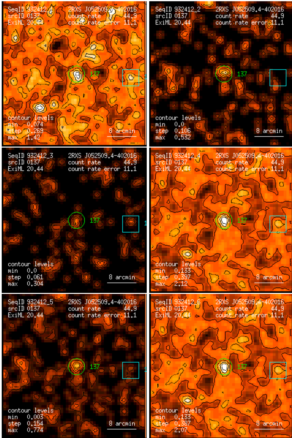
Figure 137: RASS 932412: detection 0137: band rate images, Gaussian filter: (1) PSPC channels 11 – 41, (2) 52 – 90, (3) 91 – 201, (4) 11 – 235, (5) 52 – 201, (6) 11 – 201. Broad band rates in counts/ks. Band rate contour levels in counts/ks/arcmin 2 .
