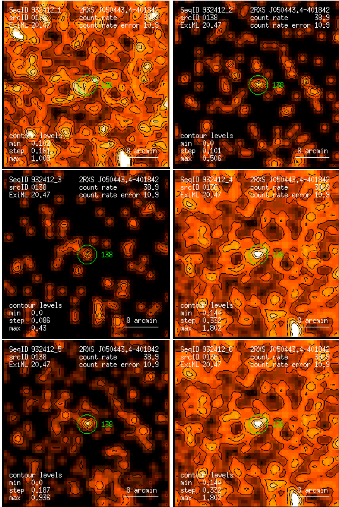
Figure 138: RASS 932412: detection 0138: band rate images, Gaussian filter: (1) PSPC channels 11 – 41, (2) 52 – 90, (3) 91 – 201, (4) 11 – 235, (5) 52 – 201, (6) 11 – 201. Broad band rates in counts/ks. Band rate contour levels in counts/ks/arcmin 2 .
