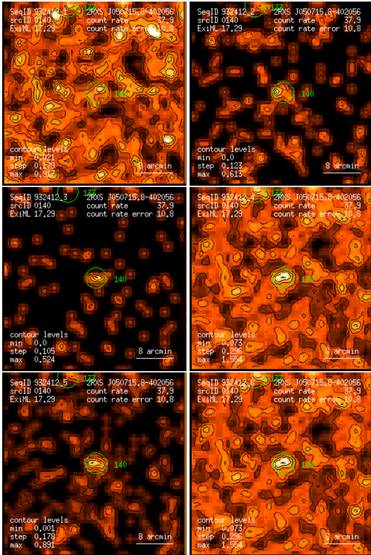
Figure 140: RASS 932412: detection 0140: band rate images, Gaussian filter: (1) PSPC channels 11 – 41, (2) 52 – 90, (3) 91 – 201, (4) 11 – 235, (5) 52 – 201, (6) 11 – 201. Broad band rates in counts/ks. Band rate contour levels in counts/ks/arcmin 2 .
