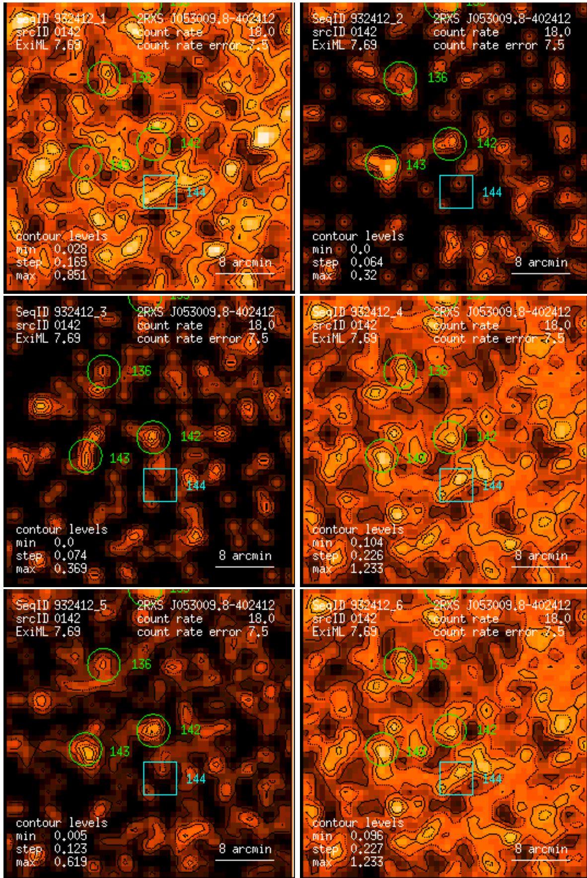
Figure 142: RASS 932412: detection 0142: band rate images, Gaussian filter: (1) PSPC channels 11 – 41, (2) 52 – 90, (3) 91 – 201, (4) 11 – 235, (5) 52 – 201, (6) 11 – 201. Broad band rates in counts/ks. Band rate contour levels in counts/ks/arcmin 2 .
