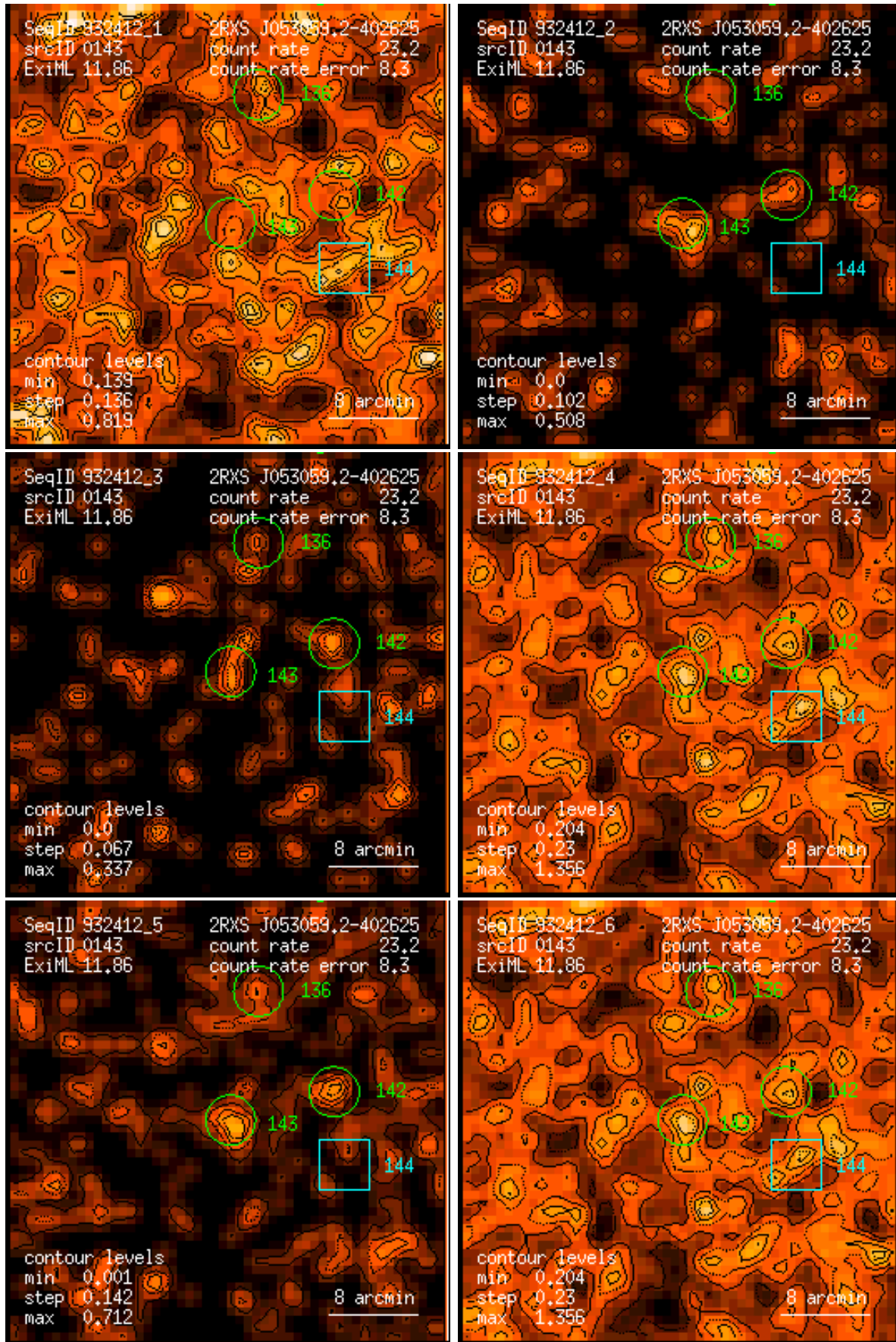
Figure 143: RASS 932412: detection 0143: band rate images, Gaussian filter: (1) PSPC channels 11 – 41, (2) 52 – 90, (3) 91 – 201, (4) 11 – 235, (5) 52 – 201, (6) 11 – 201. Broad band rates in counts/ks. Band rate contour levels in counts/ks/arcmin 2 .
