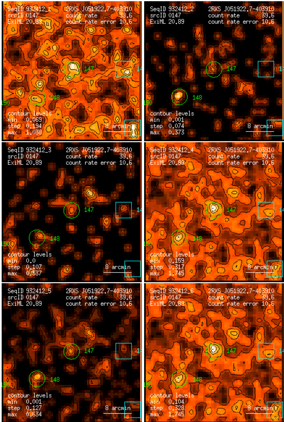
Figure 147: RASS 932412: detection 0147: band rate images, Gaussian filter: (1) PSPC channels 11 – 41, (2) 52 – 90, (3) 91 – 201, (4) 11 – 235, (5) 52 – 201, (6) 11 – 201. Broad band rates in counts/ks. Band rate contour levels in counts/ks/arcmin 2 .
