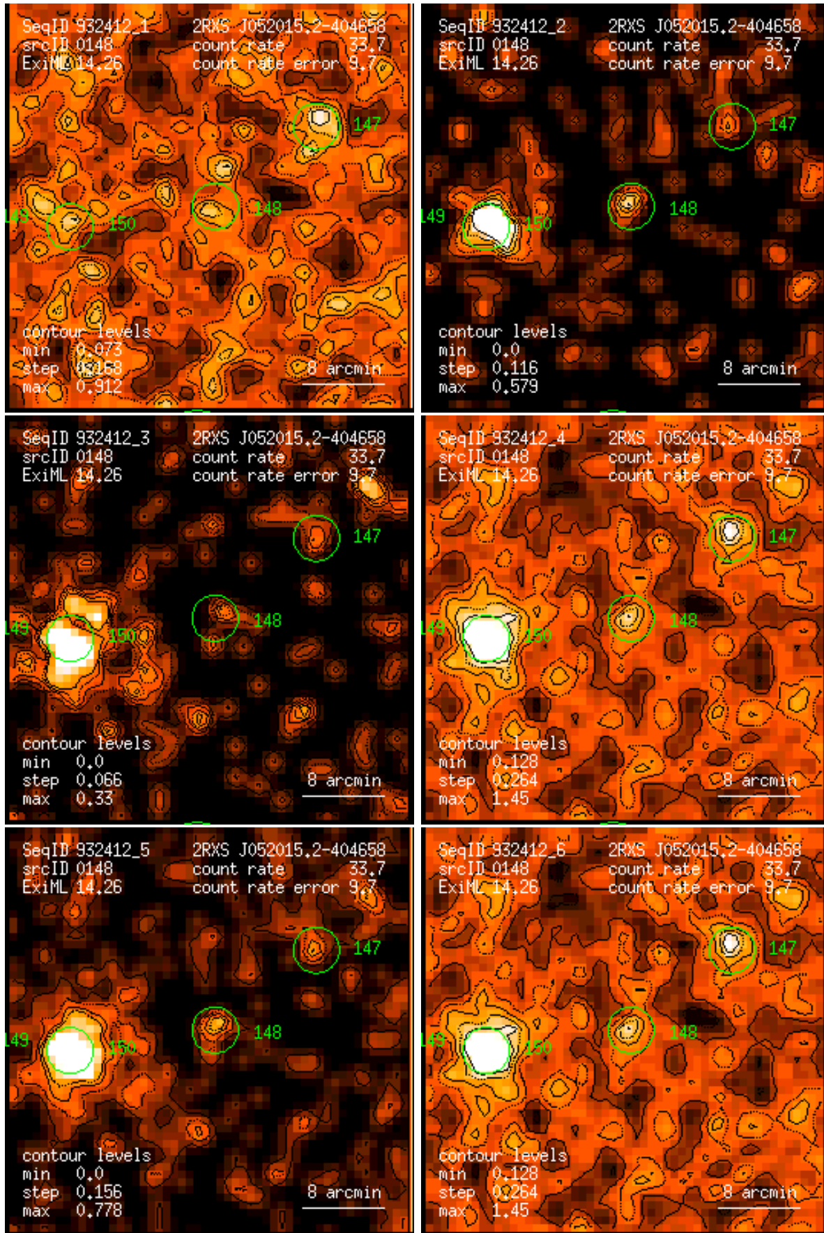
Figure 148: RASS 932412: detection 0148: band rate images, Gaussian filter: (1) PSPC channels 11 – 41, (2) 52 – 90, (3) 91 – 201, (4) 11 – 235, (5) 52 – 201, (6) 11 – 201. Broad band rates in counts/ks. Band rate contour levels in counts/ks/arcmin 2 .
