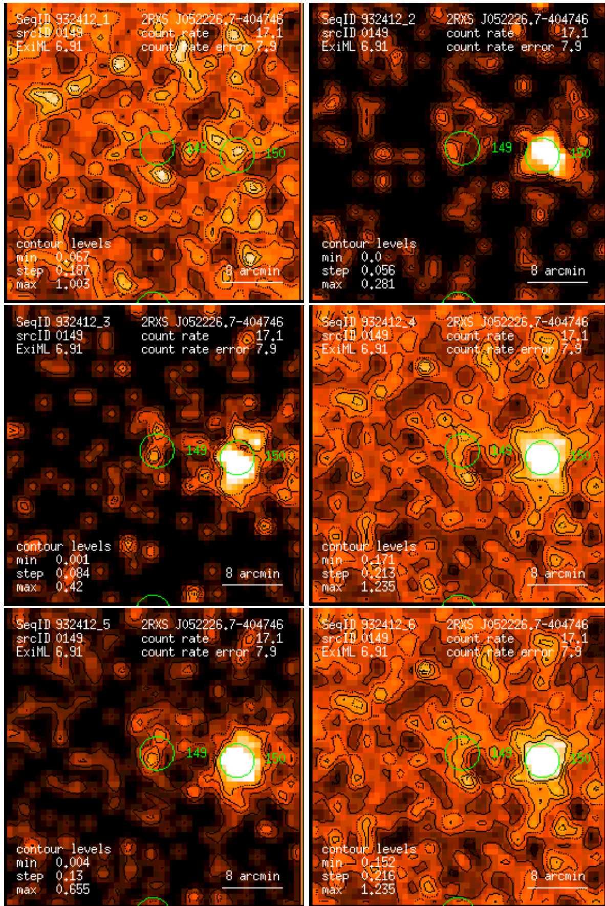
Figure 149: RASS 932412: detection 0149: band rate images, Gaussian filter: (1) PSPC channels 11 – 41, (2) 52 – 90, (3) 91 – 201, (4) 11 – 235, (5) 52 – 201, (6) 11 – 201. Broad band rates in counts/ks. Band rate contour levels in counts/ks/arcmin 2 .
