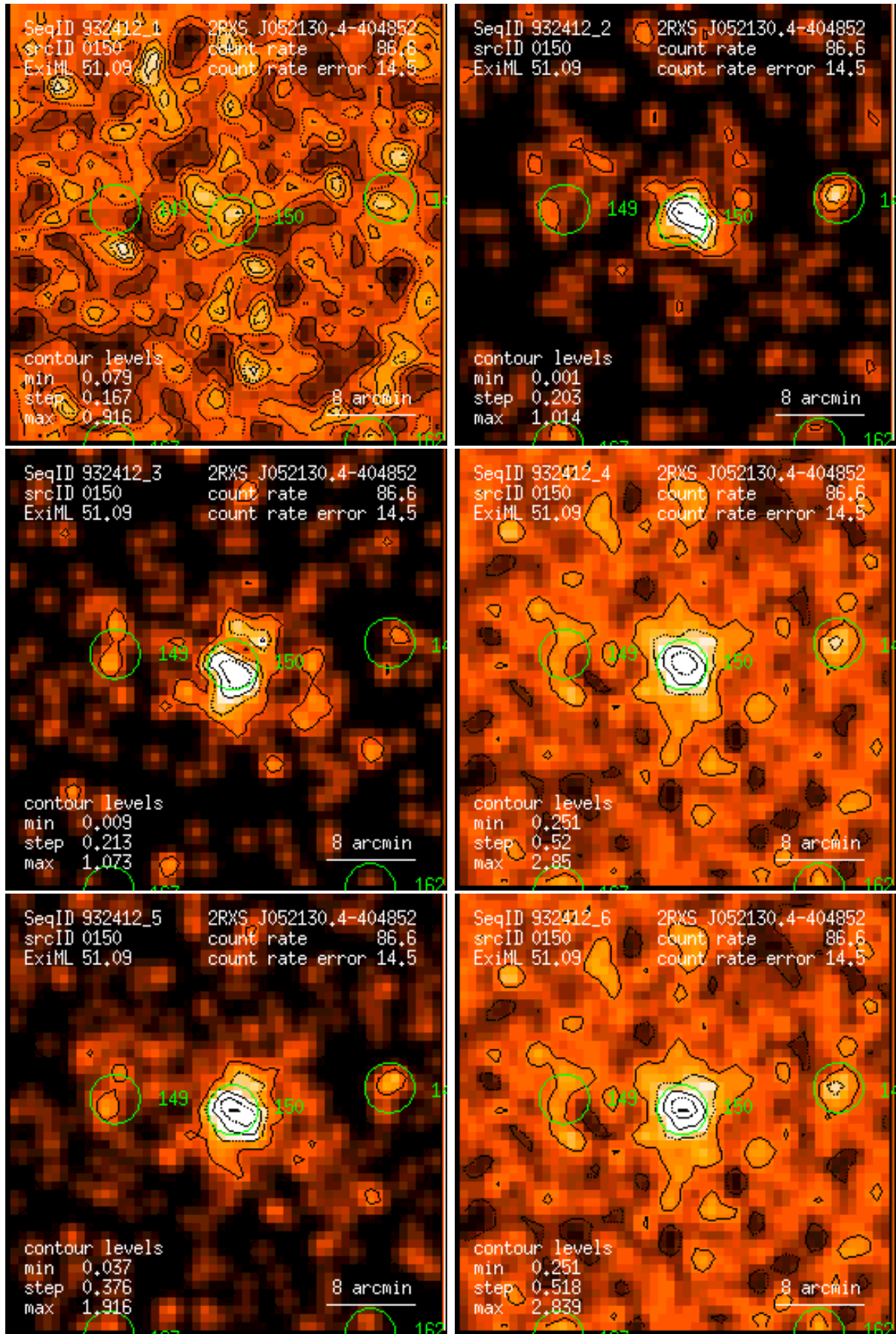
Figure 150: RASS 932412: detection 0150: band rate images, Gaussian filter: (1) PSPC channels 11 – 41, (2) 52 – 90, (3) 91 – 201, (4) 11 – 235, (5) 52 – 201, (6) 11 – 201. Broad band rates in counts/ks. Band rate contour levels in counts/ks/arcmin 2 .
