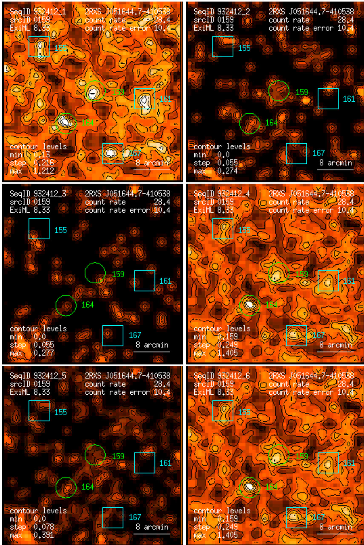
Figure 159: RASS 932412: detection 0159: band rate images, Gaussian filter: (1) PSPC channels 11 – 41, (2) 52 – 90, (3) 91 – 201, (4) 11 – 235, (5) 52 – 201, (6) 11 – 201. Broad band rates in counts/ks. Band rate contour levels in counts/ks/arcmin 2 .
