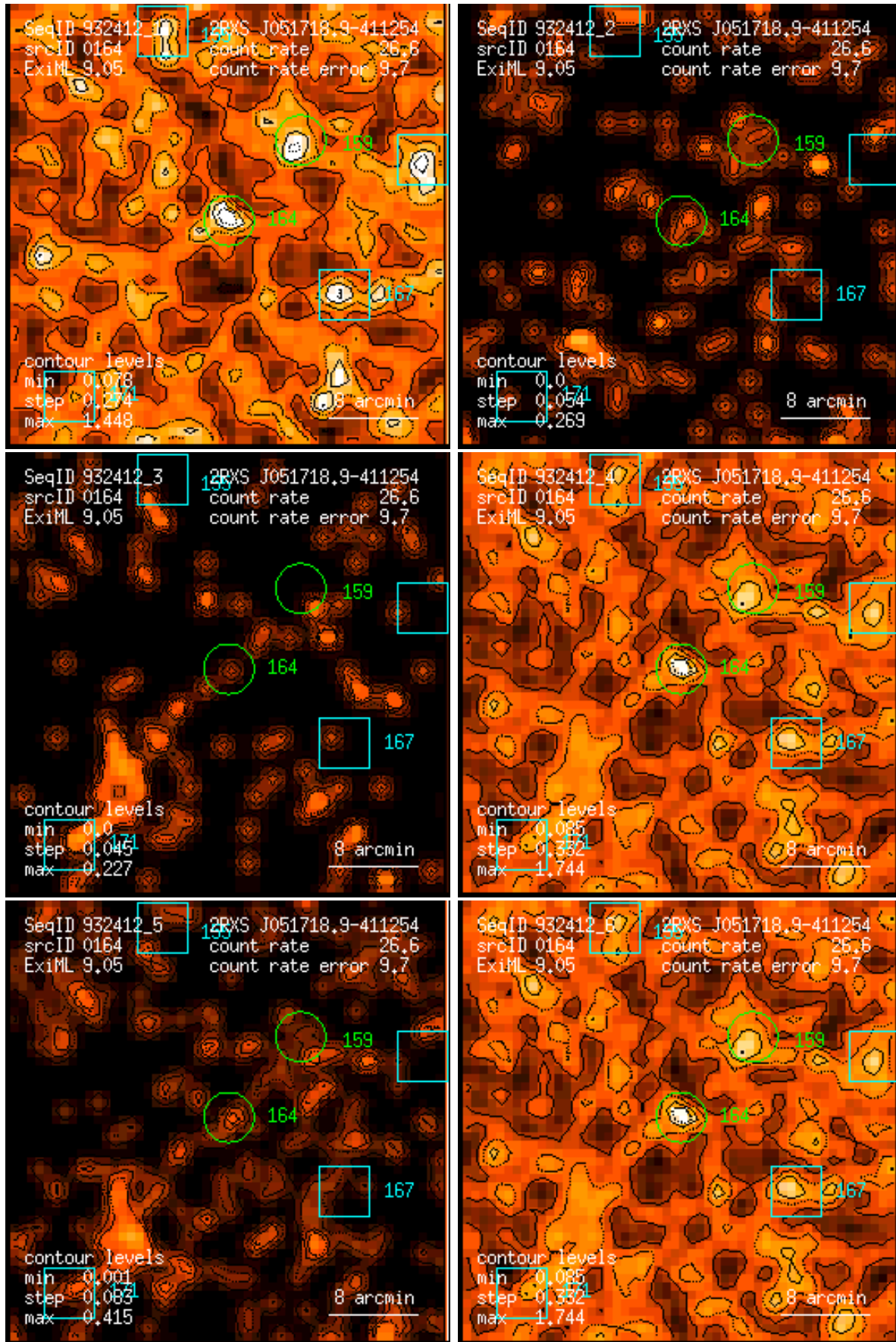
Figure 164: RASS 932412: detection 0164: band rate images, Gaussian filter: (1) PSPC channels 11 – 41, (2) 52 – 90, (3) 91 – 201, (4) 11 – 235, (5) 52 – 201, (6) 11 – 201. Broad band rates in counts/ks. Band rate contour levels in counts/ks/arcmin 2 .
